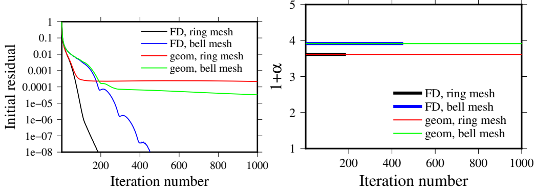
Figure 5: Convergence of initial residual of the solution of the Poisson equation for each fixed point iteration and 1 + \alpha as a function of iteration number for the planar meshes generated with the monitor function defined in eqn. (37).
