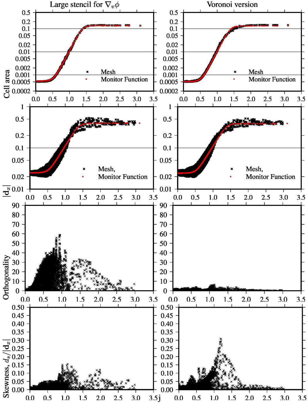
Figure 16: Mesh diagnostics as a function of distance from the centre of the refined region for the X16 meshes of 2,562 cells using the large stencil for \nabla_v \phi on the left and using the Voronoi tessellation on the right.
