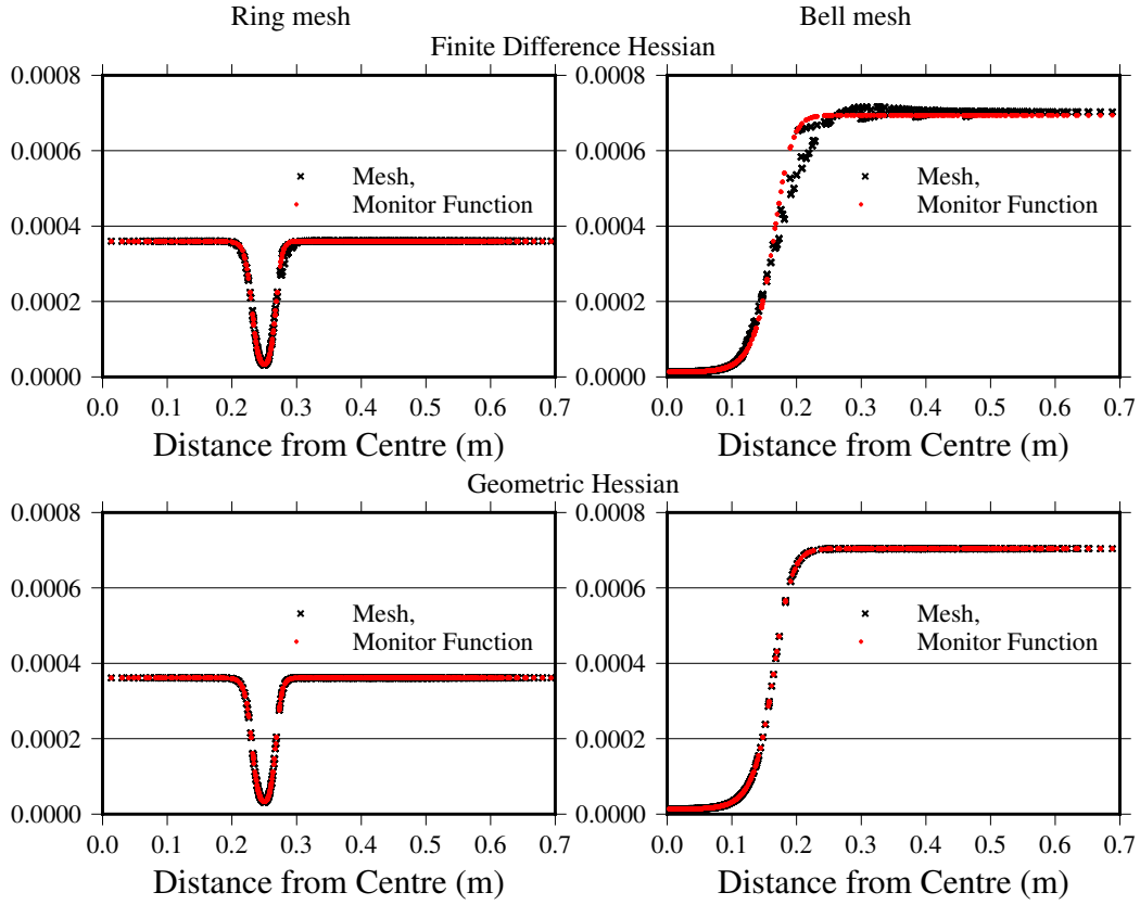
Figure 6: Cell area as a function of distance from the axis of symmetry in comparison to that implied by the monitor function ( c/m ) for the planar meshes generated with the monitor function defined in eqn. (37).
