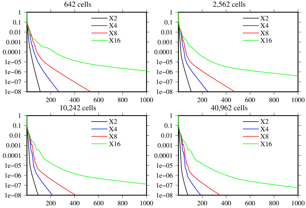
Figure 8: Convergence of initial residuals with iteration number for all of the optimally transported meshes on the sphere
