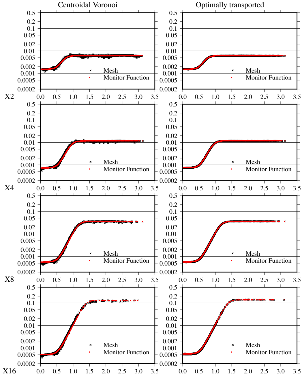
Figure 10: Cell area as a function of geodesic distance to the centre of the refined region in comparison to that implied by the monitor function ( c/m ) for the X2, X4, X8 and X16 meshes of 2,562 cells
