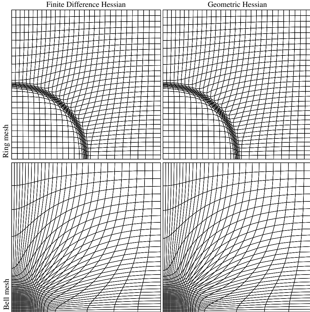
Figure 4: A quarter of the ring and bell meshes using the finite difference and volume Hesssian.
