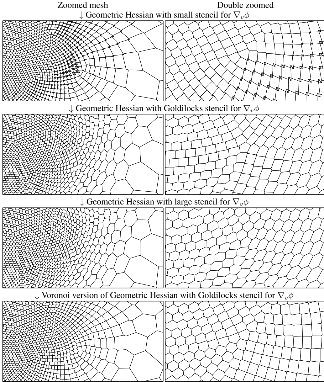
Figure 14: Zoomed and double zoomed X16 meshes with 2,562 cells using different calculations of \nabla_v \phi and Voronoi versions.
