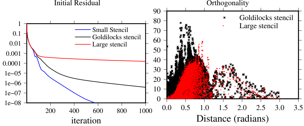
Figure 15: Comparisons of convergence of initial residuals and orthogonality for the X16 meshes of 2,562 cells calculated using the geometric Hessian but with different calculations of \nabla_v \phi .
