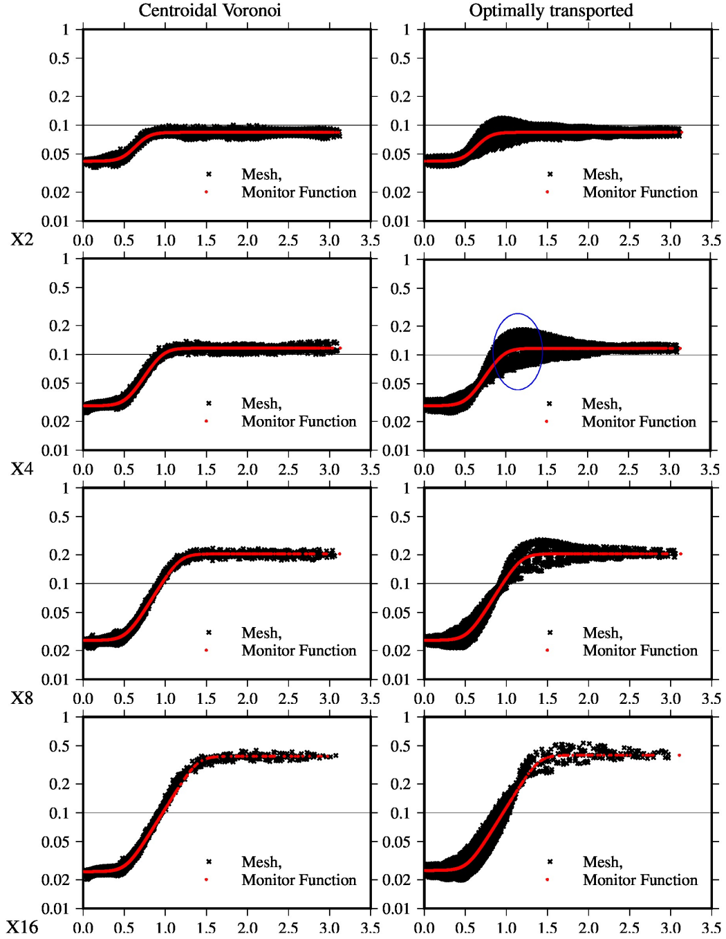
Figure 11: Cell-centre to cell-centre geodesic distance ( |d_x| as defined in section 5) as a function of geodesic distance to the centre of the refined region in comparison to that implied by the monitor function ( \sqrt{2c \tan(\pi/3)/3m} ) for the X2, X4, X8 and X16 meshes of 2,562 cells. The blue encircled region for X4 shows where the OT mesh is anisotropic.
