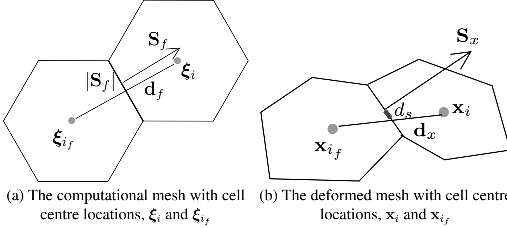
Figure 2: Cells i and i_f of the computational and deformed meshes either side of face f , face area vector \mathbf{S}_f and vector between cell centres, \mathbf{d}_f . The skewness of face f of the deformed mesh (b) is shown by a short grey line of length d_s in the plane of the face (see section 5).
