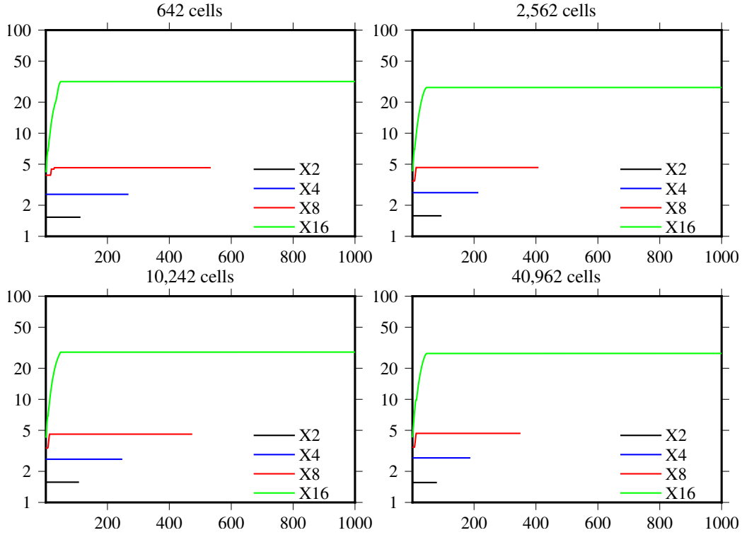
Figure 9: Under-relaxation factor, 1 + \alpha , for with iteration number for all of the optimally transported meshes on the sphere
