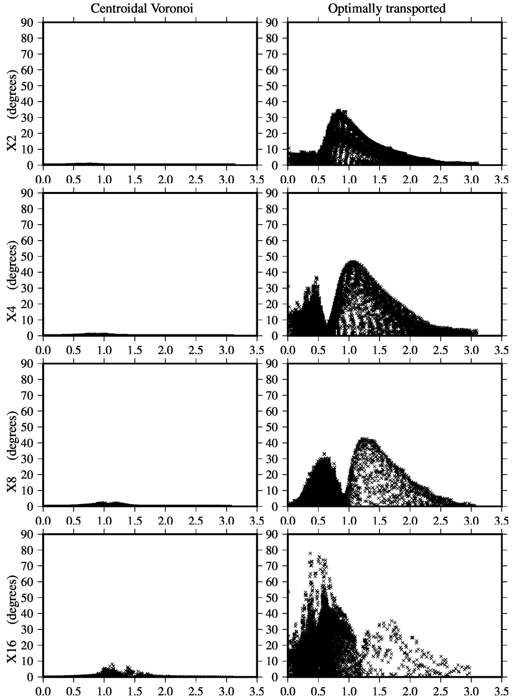
Figure 12: Non-orthogonality of the meshes on the sphere (as defined in eqn. 35) as a function of geodesic distance to the centre of the refined region for the X2-X16 meshes of 2,562 cells
