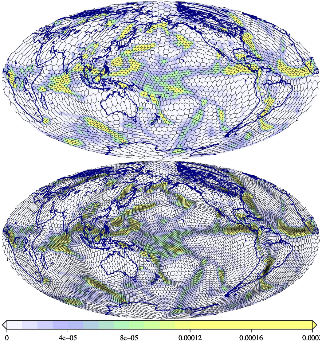
Figure 17: Meshes of 2,562 and 10,242 cells generated based on the monitor function of precipitation on 9 Oct 2012. The colours show the precipitation rate in \text{kgm}^{-2}\text{s}^{-1} . The surface of the entire sphere is displayed using a Hammer equal-area projection [42].
