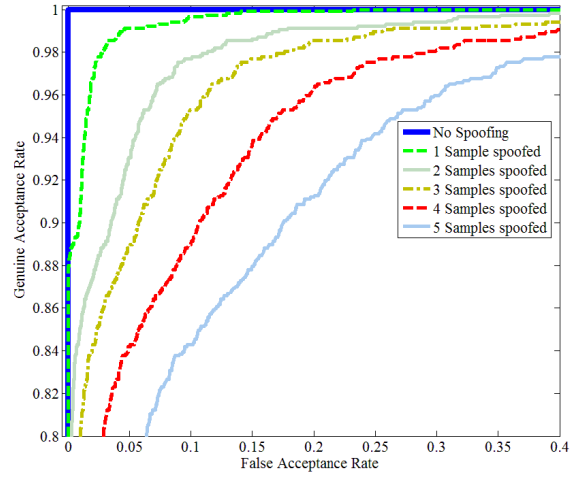
Figure 6: ROC for Partial Multibiometric Spoofing using Sum rule.
