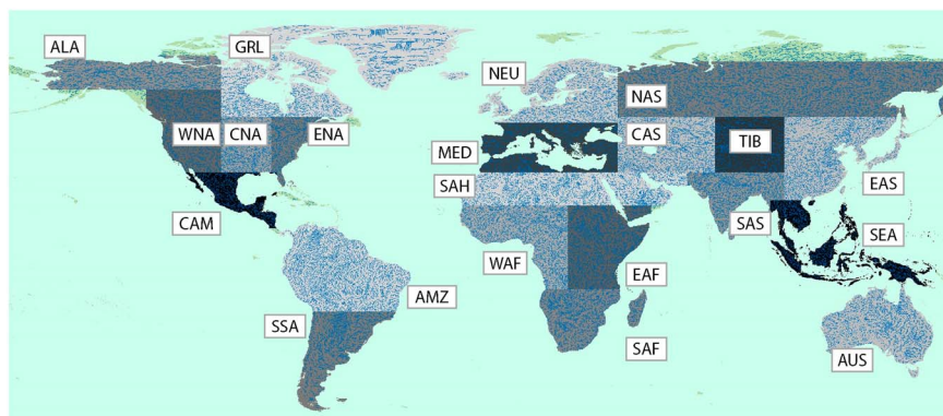
Figure 1. The GloFAS model river network, divided by the 21 regions described by Giorgi and Francisco [2000].
