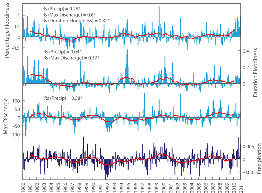
Figure 2. Time series of anomalies in monthly percentage floodiness, monthly duration floodiness, maximum monthly discharge, and mean monthly precipitation from 1980 to 2010 for all global major river pixels at 0.1° resolution. Two year running mean displayed as red line. Annotations indicate the Spearman's rank correlation coefficient, with significance at 0.05 indicated by *.
