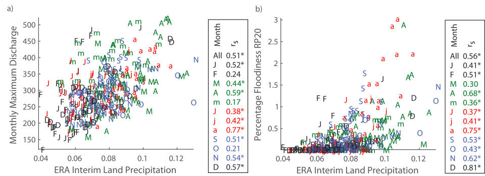
Figure 3. Correlation between (a) precipitation and discharge and the (b) percentage floodiness index for the East Africa Giorgi Region. Different months are represented by (capitalized) initials (e.g., March = M; May = m) and different seasons by colors. The legend indicates the Spearman's rank correlation coefficient, with significance at 0.05 indicated by *.
