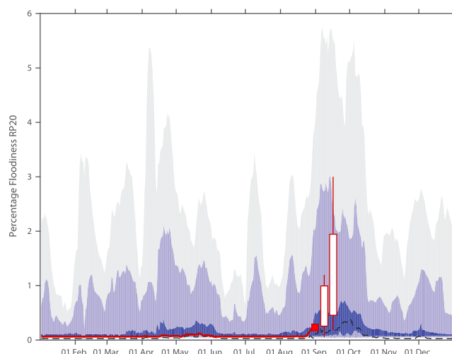
Figure 4. A climatological of 20 year return period percentage floodiness (1980–2010) for the East Africa Giorgi region. Light purple = 5th to 95th percentile, Dark purple = 33rd to 67th percentiles, Light grey = full range. A mock-up weekly floodiness forecast is shown in red.
