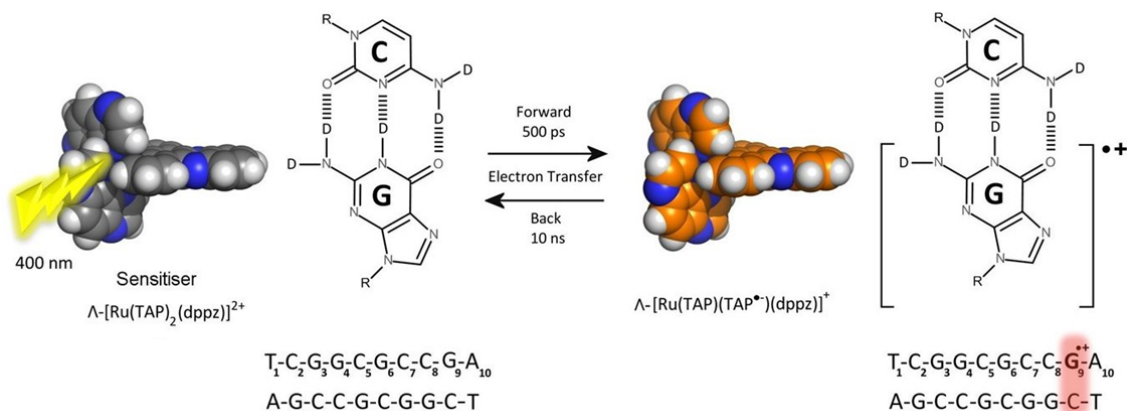
Scheme 1 | Summary of reversible oxidation of the guanine site in \Lambda\text{-}[\text{Ru}(\text{TAP})_2(\text{dppz})]^{2+} bound (TCGGCGCCGA) 2 .
