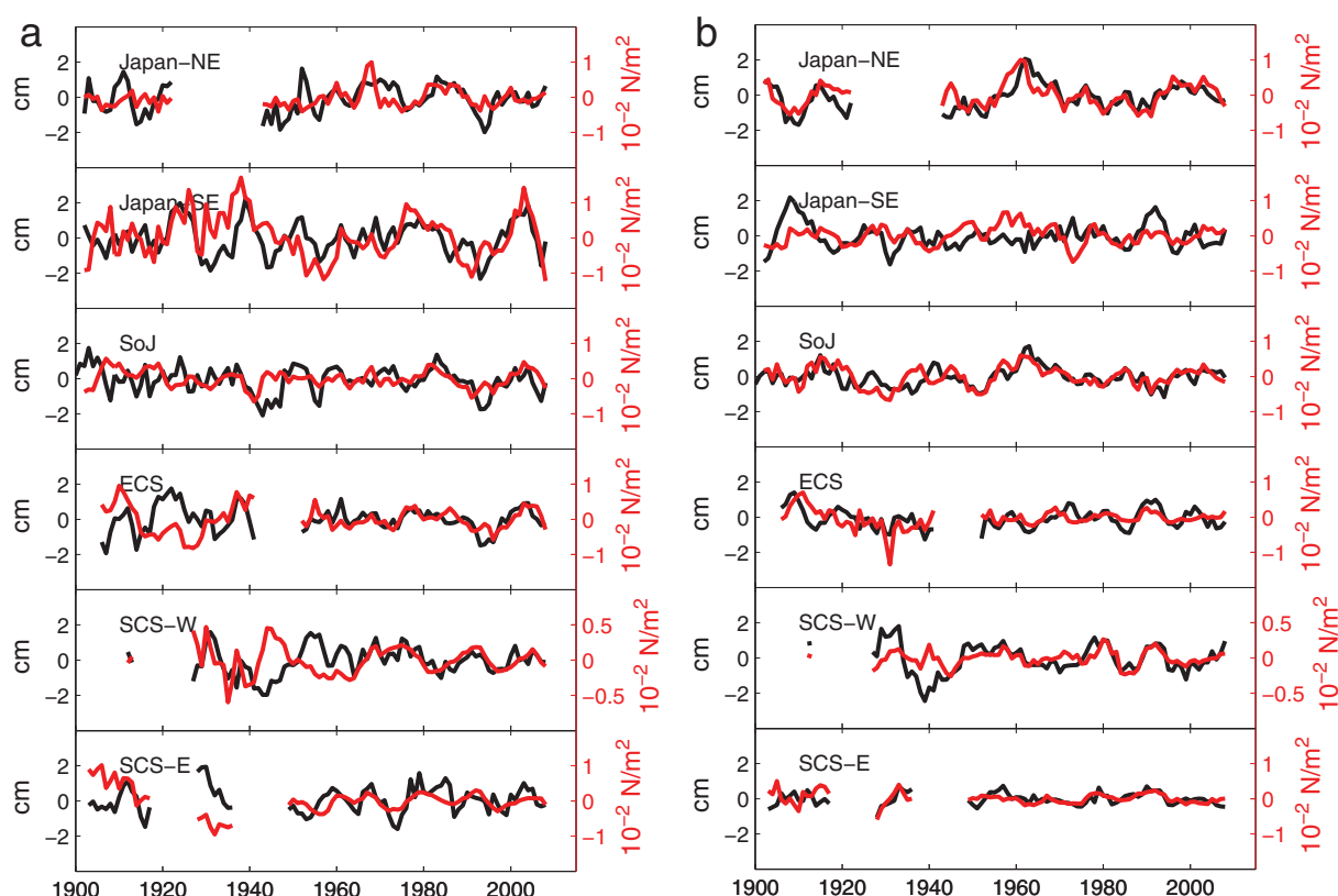
Figure 11. Time series of regional average anomaly of (a) A_a and (b) A_{sa} for \eta - \eta_{IB} (black) against the corresponding average of the wind stress (red) in six subregions as specified in Figure 1.
