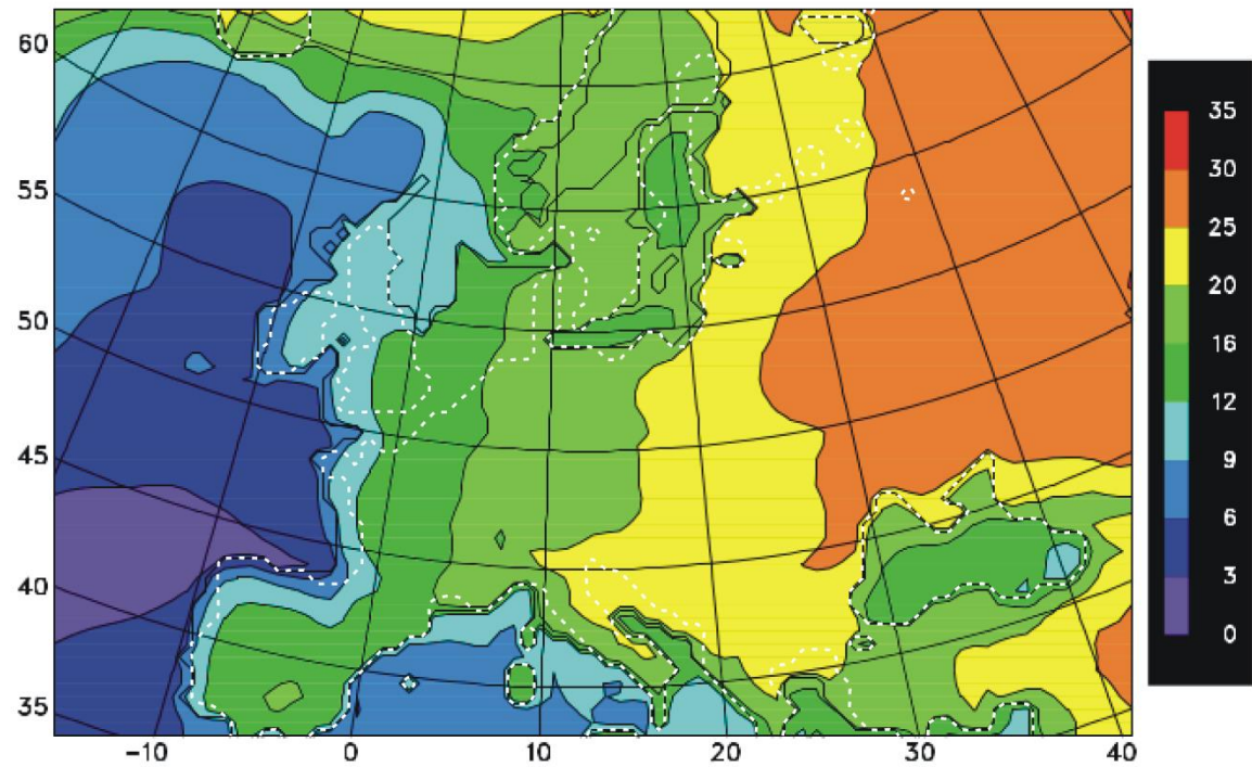
Figure 3: Summer/winter contrasts in mean air temperature data (°C) from the Stage 3 Project's MIS-3 'warm' simulation (Barron, van Andel, and Pollard 2003, appendix 5.1). Dashed white line: Modern European coastline.
