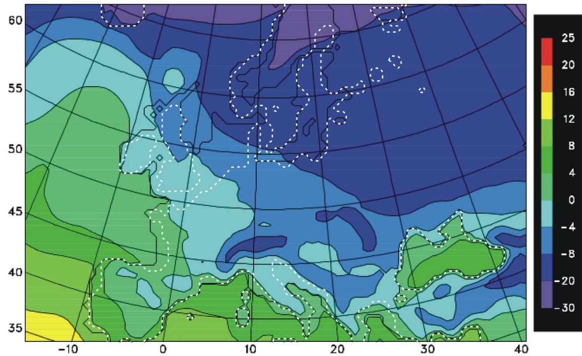
Figure 2: Mean winter air temperature data (°C) from the Stage 3 Project's MIS-3 'warm' simulation (Barron, van Andel, and Pollard 2003, fig. 5.7 [Stage 3 Warm Phase DJF]). Dashed white line: Modern European coastline.
