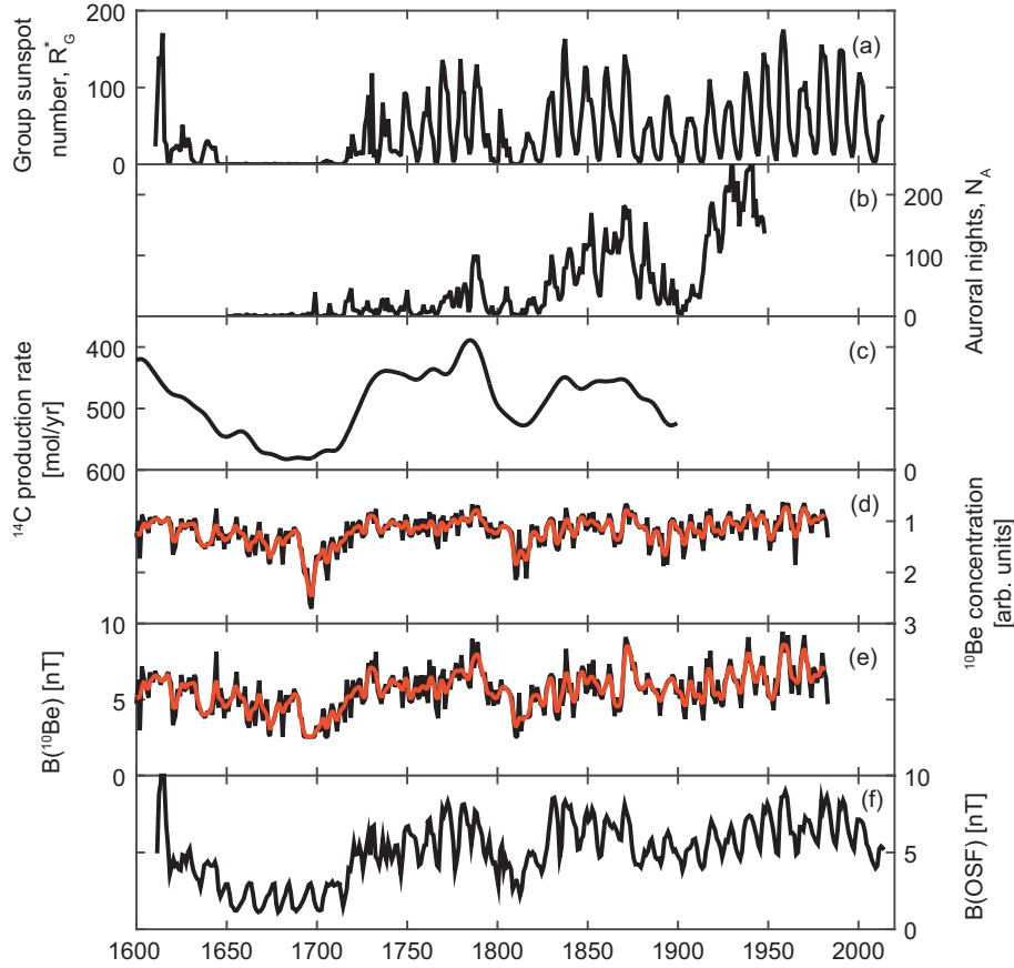
Fig. 1. Annual values of solar, GCR and heliospheric parameters from 1600 to present. (a) Corrected group sunspot number, R_G^* ; (b) Number of auroral nights below 61° geomagnetic latitude; (c) ^{14}\text{C} production rate; (d) Average concentration of ^{10}\text{Be} at annual resolution (black) and smoothed using a running 1,4,6,4,1 filter window (red); (e) near-Earth heliospheric magnetic field intensity, B , computed from ^{10}\text{Be} concentration, in the same format; (f) B estimated from the open solar flux continuity model using R_G^* . Note that the y-axis direction is inverted for panels (c) and (d), as cosmogenic isotope production falls with rising solar activity.
