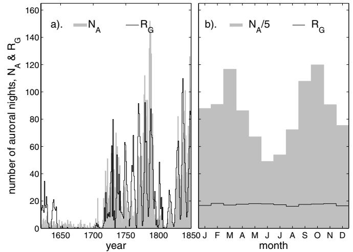
Fig. 12. Same as Fig. 10, but compiled from 41 different catalogues of auroral observations at magnetic latitudes below 55^\circ in Europe, Asia, North Africa, New England and Great Britain. The time series covers both the Maunder and the Dalton minima.
