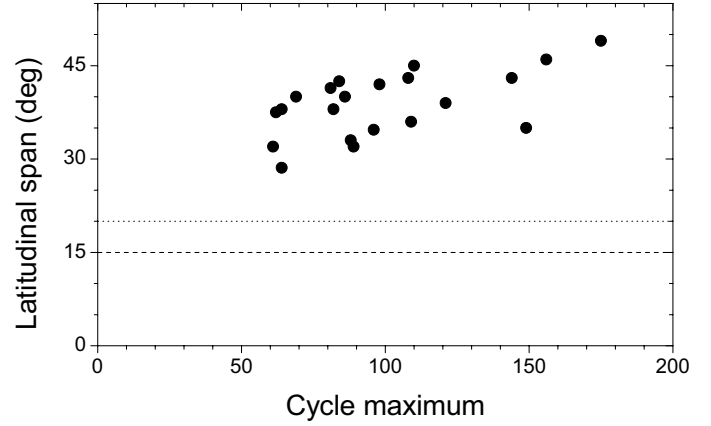
Fig. 6. Maximum latitudinal span of the butterfly diagram as a function of the cycle amplitude in annual R_G for solar cycles # 0–4 and 7–22, accounting only for large spots (with an area greater than 100 msd). The dashed and dotted lines depict the maximum latitudinal extent of sunspot occurrence during the core (1645–1700) and the entire MM (1645–1712).
