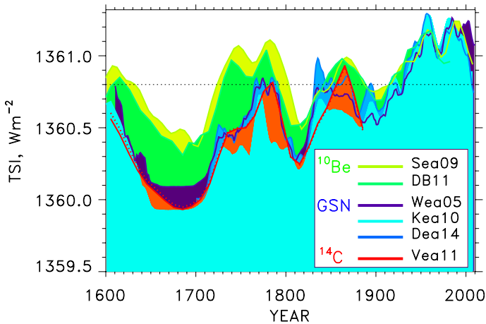
Fig. 17. Selected TSI reconstructions since 1600, labeled in the plot are: Sea09 – Steinhilber et al. (2009); DB11 – Delaygue & Bard (2011); Wea05 – Wang et al. (2005); Kea10 – Krivova et al. (2010); Dea14 – Dasi-Espuig et al. (2014, priv. comm.); Veal1 – Vieira et al. (2011). The green, blue and red colour tones are used for the reconstructions based on the ^{10}\text{Be} , sunspot and ^{14}\text{C} data, respectively. The black dotted line marks the TSI value at modern solar activity minimum conditions according to SORCE/TIM measurements.
