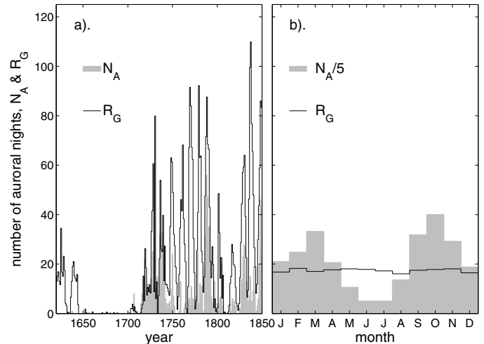
Fig. 10. Panel A) number of auroral nights, N_A , in calendar years for observations in Great Britain collated by E. J. Lowe (1870) with the addition of the observations by Thomas Hughes (Harrison 2005) and John Dalton (Dalton 1834) (grey histogram). Annual group sunspot number of Hoyt & Schatten (1998), with the adoption of recent corrections by Vaquero et al. (2011) and Vaquero & Trigo (2014) (black line). Lowes personal copy of his catalogue of natural phenomena (including auroras) was only recently discovered and was compiled completely independently of other catalogues. Yet it shows, like the others, the dearth of sightings during the MM, some events in 1707 and 1708 and the return of regular sightings in 1716. Panel B) annual variation of N_A in the same dataset and of R_G .
