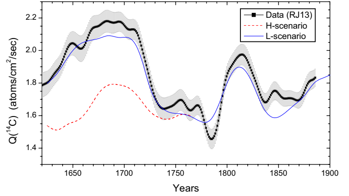
Fig. 14. Time profile of decadal smoothed radiocarbon ^{14}\text{C} production rate. The black curve with grey error bars represents the reconstruction by Roth & Joos (2013) based on the Intcal13 (Reimer et al. 2013) radiocarbon data. Coloured curves depict the computed production for the two scenarios as labeled in the legend (see text for details).
