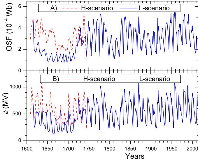
Fig. 13. Evolution with time of the open solar magnetic flux, OSF, (panel A) and of the modulation potential \phi (panel B) for the two scenarios of solar activity during the MM (see text).
