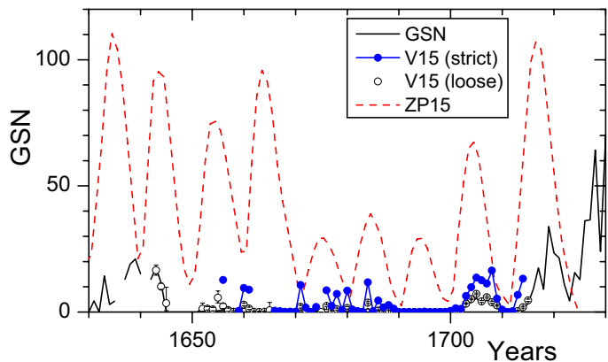
Fig. 1. Annual group sunspot numbers during and around the Maunder minimum, according to Hoyt & Schatten (1998) – GSN, Zolotova & Ponyavin (2015) – ZP15, and loose and strictly conservative models from Vaquero et al. (2015a) (see Sect. 2.1), as denoted in the legend.
