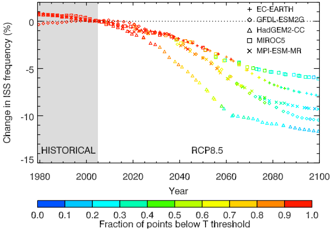
Figure 6. Time series of the change in 250 hPa CISS frequency (in percentage points) in the tropics in the CMIP5 models (symbols) from 1979 to 2099, calculated for each year as the annual-mean CISS frequency minus the 1979–2005 average (the historical period, shown by grey shading). The colour of the points shows the fraction of points in the tropics which are below the 233 K temperature threshold for CISS. A 10-year running mean has been applied to each time series before plotting.
