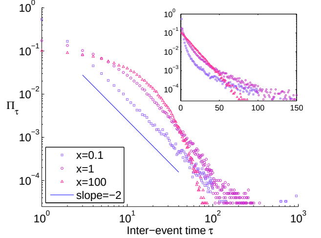
FIG. 3. (Colour online) The inter-event time distribution for attachment events of a single node i with fitness equal to the mean of the fitness distribution ( x_i = \langle x \rangle ) on Log-Log axes (main), and Log-Linear axes (inset). The plotted results consider a dense network where N = 10 and E = 100 . The attachment events of i are described by the process introduced in Section II with M=E and \epsilon = (N/2 - 1)\langle x \rangle . When x_i , and hence N\langle x \rangle , are very large, the event probability is dominated by the contribution from x_i and is therefore weakly dependent on the memory of i . In this case the inter-event times are distributed exponentially (as expected in a Bernoulli process). As \langle x \rangle \rightarrow 0 the contribution from the memory of previous events becomes dominant and the distribution approaches a power-law with exponent -2 .
