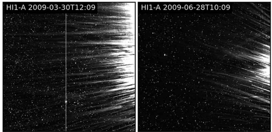
4 These two background-subtracted HI1-A images are examples of how the secondary particle trails appear as they propagate across the HI field of view.
