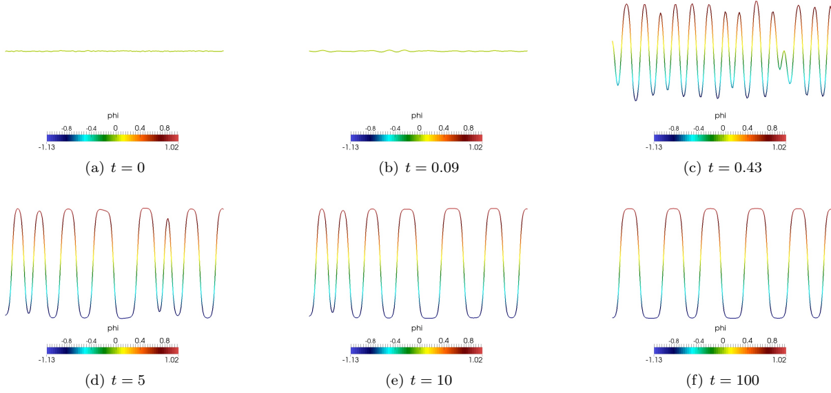
FIGURE 6. 6.11 Test 6 – As Figure 5 but in this case \rho_2/\rho_1 = 10 and \max \phi = 1.0233 hence \rho(\phi) > 0 for all time.
