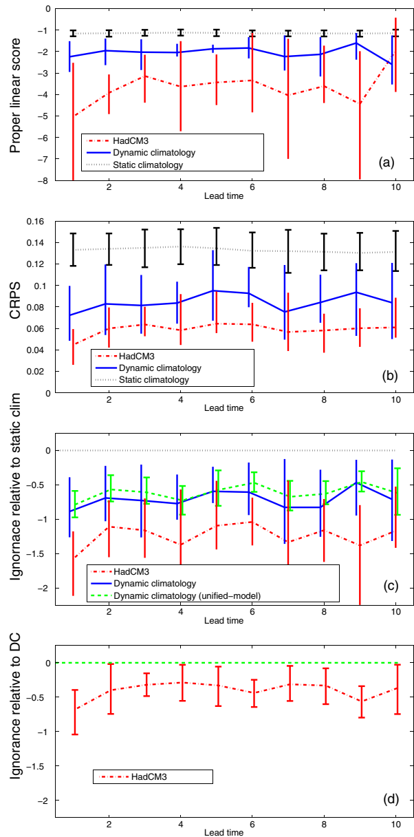
Fig. 3 Performance of HadCM3 and DC forecast systems as a function of lead time under different skill scores: a PL score, b CRPS, c IGN relative to the Static Climatology and d IGN relative to DC. In panels a , b , and c the Static Climatology (SC) is shown for comparison; in panel c both HadCM3 and DC perform substantially better than SC on average; multiple-realization sample bars ( vertical bars , no caps) show that this is the case in almost every realization. A unified DC forecast system ( green dashed ) is shown for comparison; traditional (10 %–90 %) bootstrap resample ranges ( green dashed, with caps ) reveal a similar result with somewhat improved sampling uncertainty. In Panel d the red dash-dotted line fluctuates between -0.25 bit to -0.75 bit indicating that on average the HadCM3 forecast system clearly outperforms the unified DC, placing between \sim 20\% and 60\% more probability on the outcome than DC at various lead times. Some of the multiple-realization sample bars ( no caps ) reach zero in panel ( d ), indicating that in some realizations the DC outperforms HadCM3
