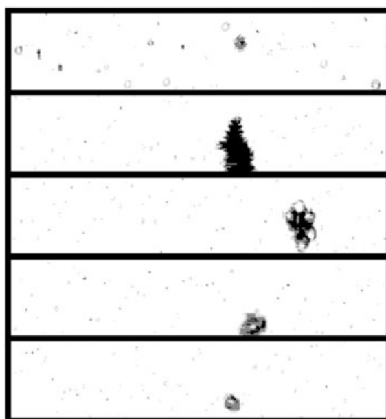
Figure 4. Example images of large dust particles collected by the CIP15 probe during flight B601. The image resolution is 15 μm, and the height of each strip is 960 μm. Note that the CIP only records pixels when a particle is in the field of view so horizontal spacing in the images is not representative of actual particle spacing.
