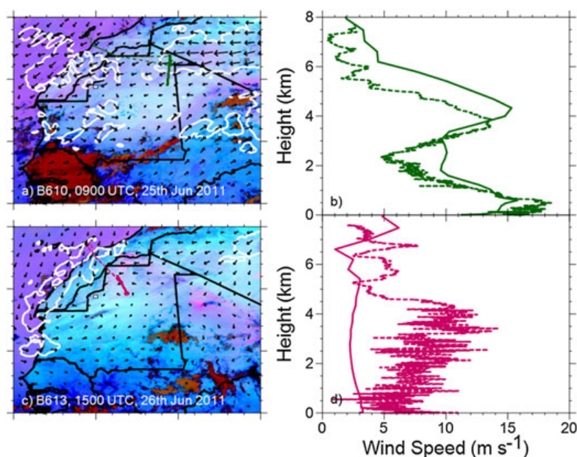
Figure 3. (a and c) Images show false color SEVIRI images overlain with forecast Africa LAM wind vectors and the white 8 m s -1 contour as per Figure 2, for times corresponding to flights B610 and B613. Colored lines show aircraft tracks as per Figure 1. (b and d) Images show forecast Africa LAM wind profiles at the same times as Figures 3a and 3c, respectively, with corresponding measured wind profile from the aircraft descents.
