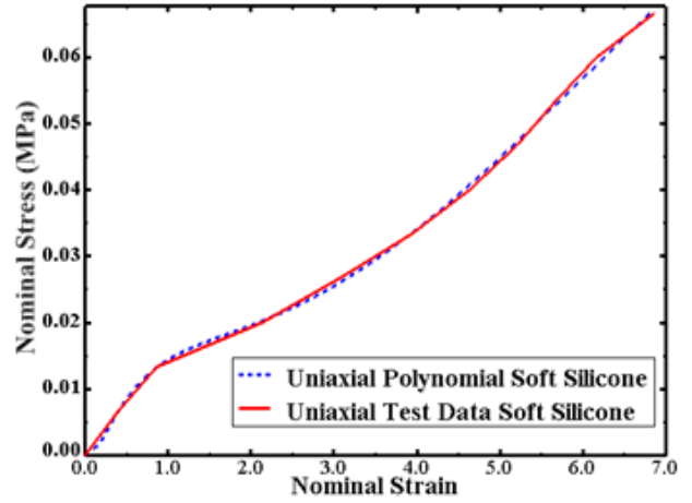
Figure 10. Strain curves of Ecoflex 0030 Silicone (Experimental and Polynomial model data)
