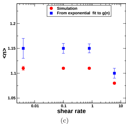
FIG. 3. For weak dipolar interaction strength \lambda \approx 2.37 : (a) the cluster size distribution g(n) as a function of chain size n for various shear rates and the exponential fit is shown as dashed line (b) The connectivity C(n_c) as a function of coordination number n_c for various shear rates (c) average chain size \langle n \rangle as a function of shear rate. Explanation given in Sec. IV A.
