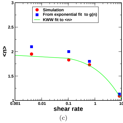
FIG. 4. For intermediate dipolar interaction strength \lambda \approx 4.62 : (a) the cluster size distribution g(n) as a function of chain size n for various shear rates and the exponential fit to the data is shown as dashed line (b) The connectivity C(n_c) as a function of coordination number n_c for various shear rates (c) average chain size \langle n \rangle as a function of shear rate. Explanation given in Sec. IV B.
