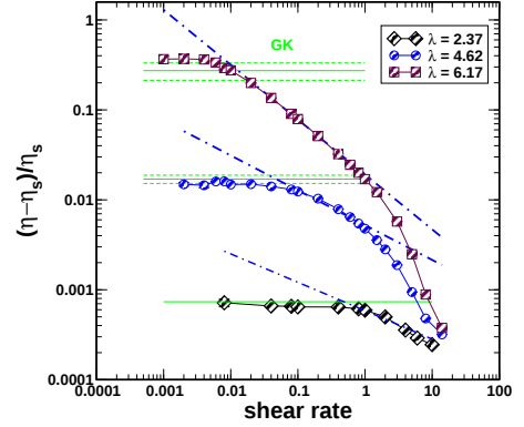
FIG. 2. The zero shear viscosity scaled by solvent viscosity as a function of shear rate for different dipolar interaction strengths ( \lambda ). A clear transition from Newtonian regime to shear thinning regime with increasing shear rate is observed. The horizontal continuous lines are equilibrium viscosities obtained from the Green-Kubo (GK) method [24] and dashed lines are error bars of equilibrium viscosities.
