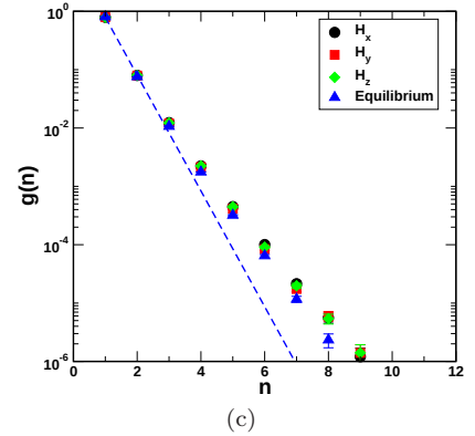
FIG. 7. For \lambda \approx 2.37 with applied field H in Newtonian regime: (a) The configurational viscosity \eta_{\text{conf}} , the rotational viscosity \eta_{\text{rot}} and the total viscosity \eta_{\text{tot}} = \eta_{\text{conf}} + \eta_{\text{rot}} as a function of strength of the magnetic field H are shown as circles, squares and diamond symbols, respectively. Top panel: Viscosities when the field is oriented in the flow direction, middle panel: when the field is oriented in the gradient of the flow direction, bottom panel: when the field is oriented in the vorticity direction. (b) The connectivity C(n_c) as a function of n_c for different orientations of magnetic field (c) Cluster size distribution g(n) as a function of n at different orientations of magnetic field. Exponential fit to g(n) is shown as dashed lines. All structural analysis are performed with a fixed magnetic field strength of H = 2.0 . Explanation is given in Sec. V A 1.
