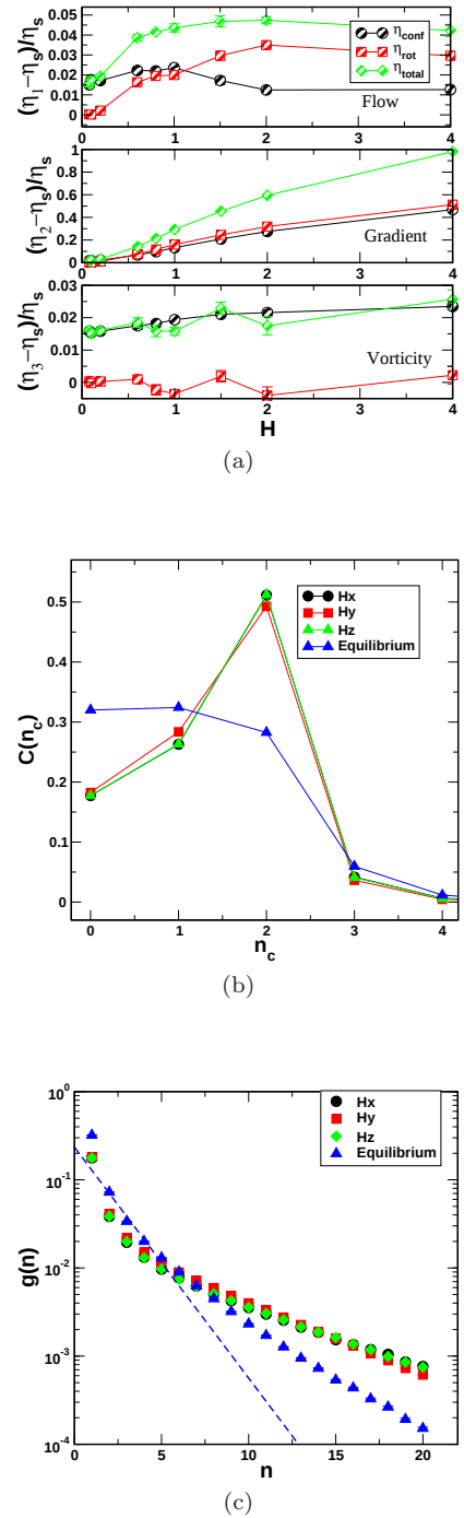
FIG. 8. For \lambda \approx 4.62 with applied field H in Newtonian regime: (a) The configurational viscosity \eta_{\text{conf}} , the rotational viscosity \eta_{\text{rot}} and the total viscosity \eta_{\text{tot}} = \eta_{\text{conf}} + \eta_{\text{rot}} as a function of strength of the magnetic field H are shown as circles, squares and diamond symbols, respectively. Top panel: Viscosities when the field is oriented in the flow direction, middle panel: when the field is oriented in the gradient of the flow direction, bottom panel: when the field is oriented in the vorticity direction. (b) The connectivity C(n_c) as a function of n_c for different orientations of magnetic field (c) Cluster size distribution g(n) as a function of n at different orientations of magnetic field. Exponential fit to the data is shown as dashed lines. All structural analysis is performed with a fixed magnetic field strength of H = 2.0 . Explanation is given in Sec. V A 2.
