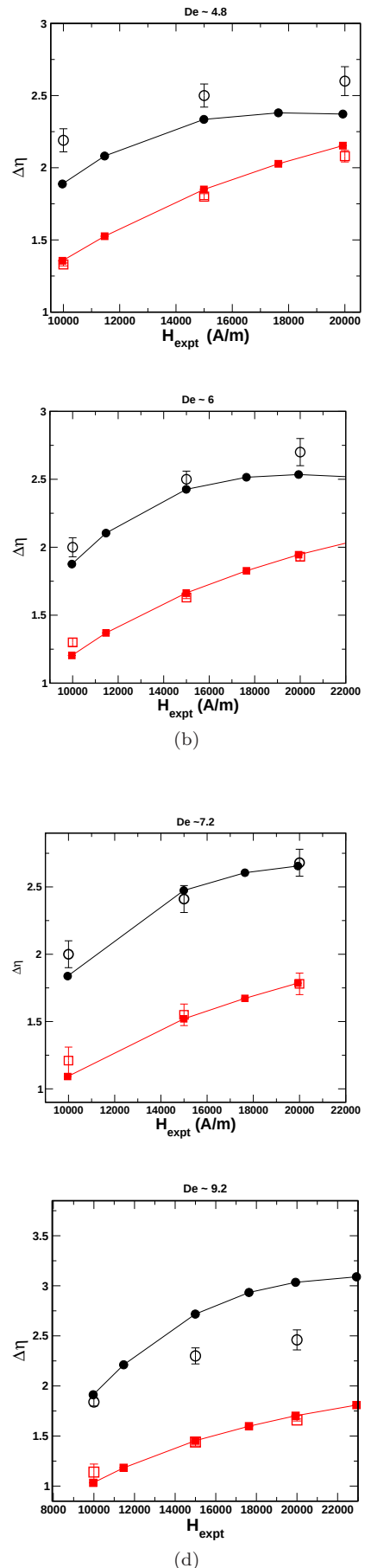
FIG. 18. The magnetoviscous effect \Delta\eta for a range of dimensionless shear rates as a function of magnetic field strength (in real units) is computed from simulations (solid symbols) and compared with experiments (open symbols). \Delta\eta_{\parallel} (circles) is the magnetoviscous effect when the field is parallel to the flow and \Delta\eta_{\perp} (squares) is the magnetoviscous effect when the field is perpendicular to the flow direction (see Eq. (11)).
