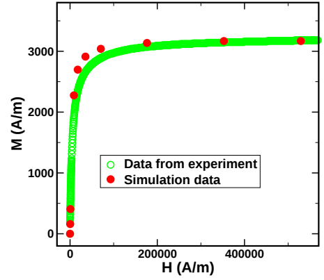
FIG. 1. The equilibrium magnetisation curve ( M ) as a function of applied magnetic field strength ( H ).
