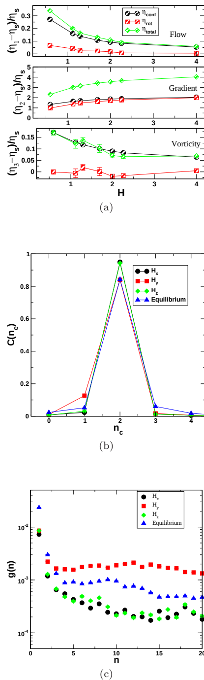
FIG. 9. For \lambda \approx 6.17 with applied field H in Newtonian regime: (a) The configurational viscosity \eta_{\text{conf}} , the rotational viscosity \eta_{\text{rot}} and the total viscosity \eta_{\text{tot}} = \eta_{\text{conf}} + \eta_{\text{rot}} as a function of strength of the magnetic field H are shown as circles, squares and diamond symbols, respectively. Top panel: Viscosities when the field is oriented in the flow direction, middle panel: when the field is oriented in the gradient of the flow direction, bottom panel: when the field is oriented in the vorticity direction. (b) The connectivity C(n_c) as a function of n_c for different orientations of magnetic field (c) Cluster size distribution g(n) as a function of n at different orientations of magnetic field. Exponential fit to the data is given as dashed line. All structural analysis are performed with a fixed magnetic field strength of H = 2.0 . Explanation is given in Sec. V A 3.
