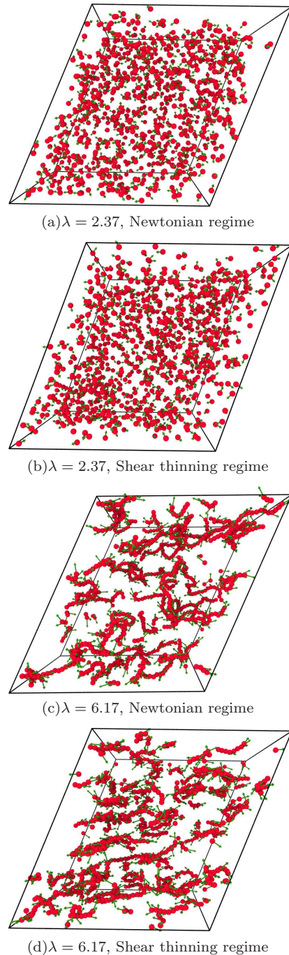
FIG. 6. Snapshots (projection of all particles) of model ferrofluid system in a shear flow in the absence of magnetic field ( H = 0 ).
