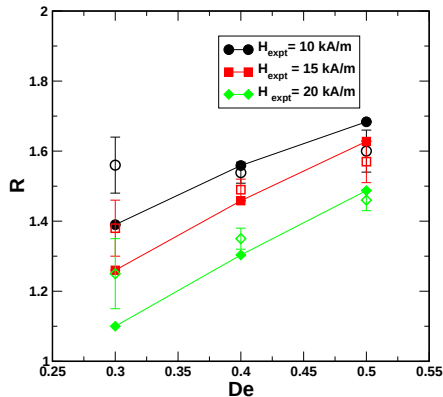
FIG. 19. The ratio R of \Delta\eta_{||} and \Delta\eta_{\perp} as a function of dimensionless shear rate for different magnetic field strengths (solid and open symbols correspond to simulation and experiment, respectively).
