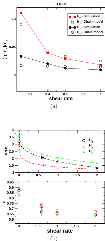
FIG. 14. For \lambda \approx 4.62 : (a) The total viscosities in the flow (circles) and gradient direction of the flow (squares) from simulations (solid symbols) and the chain model prediction (open symbols computed by inputting the values of the chain size distribution from simulations) as a function of shear rate. (b) Top panel: Average cluster size as a function of shear rate. The stretched exponential fit is shown as dashed lines. Bottom panel: The rigidity exponent \nu is shown for different orientation of magnetic field as a function of shear rate for the magnetic field strength H = 2.0 .
