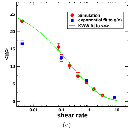
FIG. 5. For strong dipolar interaction strength \lambda \approx 6.17 : (a) the cluster size distribution g(n) as a function of chain size n for various shear rates (b) The connectivity C(n_c) as a function of coordination number n_c for various shear rates (c) average chain size \langle n \rangle as a function of shear rate. Explanation given in Sec. IV C.
