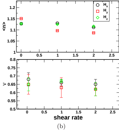
FIG. 12. For \lambda \approx 2.37 : (a) The total viscosities in the flow (circles) and gradient direction of flow (squares) from simulation (solid symbols) and the chain model prediction (open symbols computed by inputting value for chain size distribution from simulations) as a function of shear rate. (b) Top panel: Average cluster size as a function of shear rate. Bottom panel: The rigidity exponent \nu is shown for different orientation of magnetic field as a function of shear rate for the magnetic field strength H = 2.0 .
