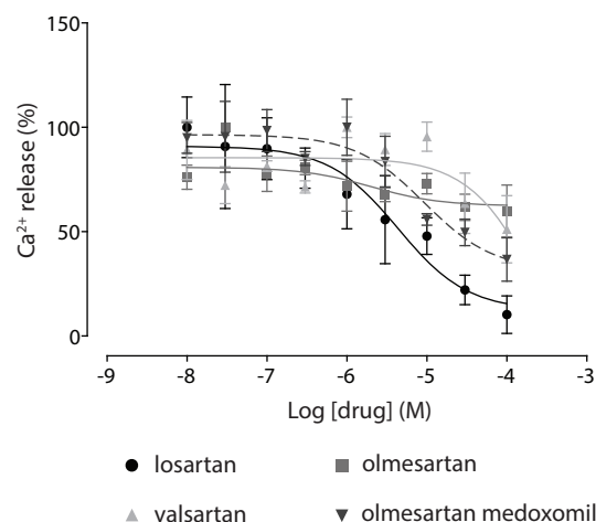
Figure 6. GPVI antagonism is unique to losartan amongst the sartan drug class. Inhibition of collagen-induced Ca^{2+} release (10 μg/ml) the sartans from fura2-AM-loaded washed human platelets was measured and quantified ( n = 3 , \pm SEM). doi:10.1371/journal.pone.0101209.g006
