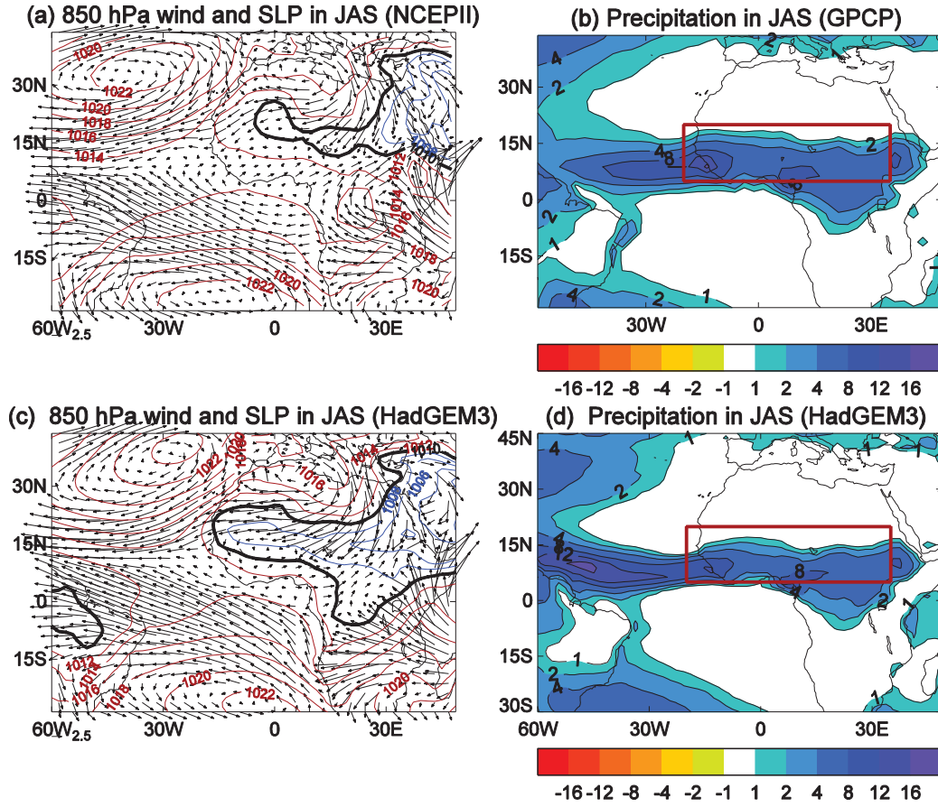
Figure S5. The spatial patterns of JAS climatology for observations and model simulation. a-b, SLP (hPa) and 850 hPa winds (m s -1 ) for NCEP reanalysis 2, and precipitation (mm day -1 ) for GPCP v2.2 (1979-2011). c-d, The same as in a-b but for the model CONTROL experiment.
