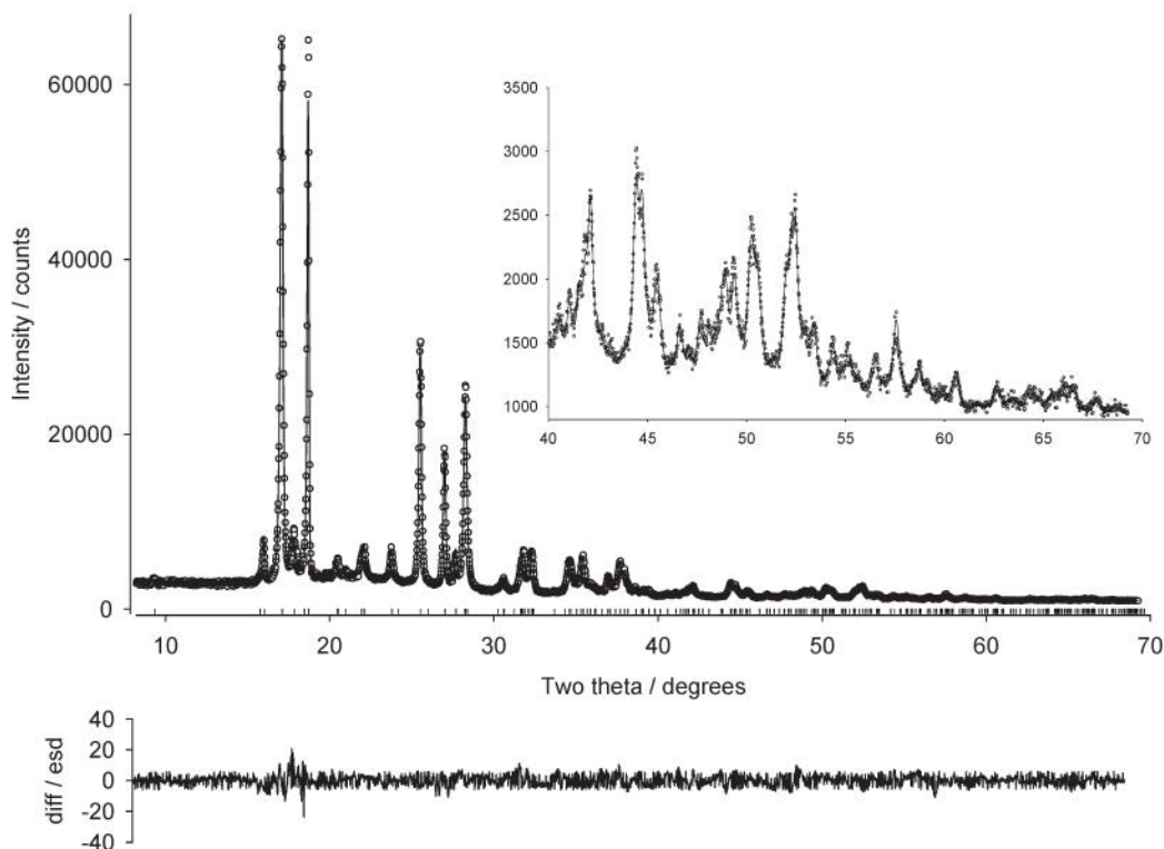
Fig. 3 Final observed (points) and calculated (line) and difference [(y_{\text{obs}} - y_{\text{cal}})/\sigma(y_{\text{obs}})] profiles for the restrained Rietveld refinement of CTN II.
