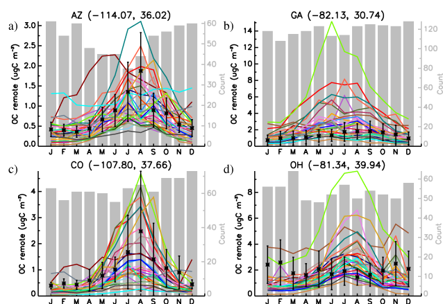
Figure 17. Same as in Fig. 16, for remote stations. Arizona (a; 114.07° W, 36.02° N, years 2000–2006); Georgia (b; 82.13° W, 30.74° N, years 1993–2006); Colorado (c; 107.80° W, 37.66° N, years 2000–2006); Ohio (d; 81.34° W, 39.94° N, years 1998–2004).
