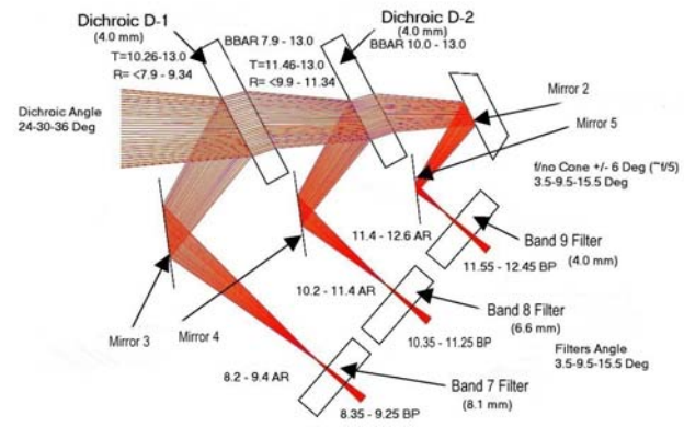
Fig 2. MSI integrated bandpass filter, dichroic and mirrors assembly coating layout
