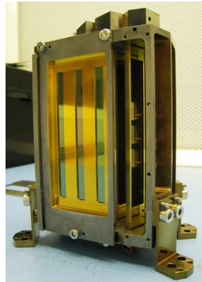
Fig 4. Manufactured filter and dichroic optical assembly
