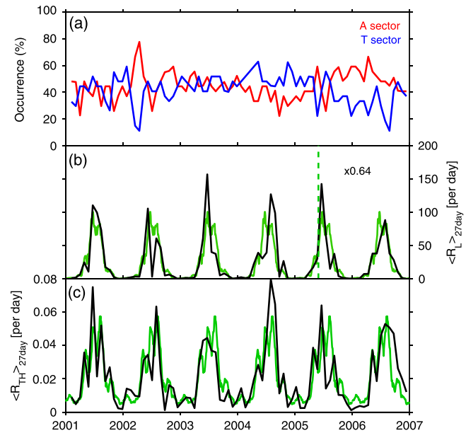
Figure 1. Time series of the datasets used in this study. (a) The percentage occurrence of away (A, red) and toward (T, blue) heliospheric magnetic field sectors. (b) R_L , the daily UK lightning stroke rate from the ATD radio network (black) and its mean seasonal variation (green). (c) R_{TH} , UK thunder day rate (black) and its mean seasonal variation (green). All data have been 27 day averaged for purposes of plot clarity, but all analysis in this study is performed on daily data.
