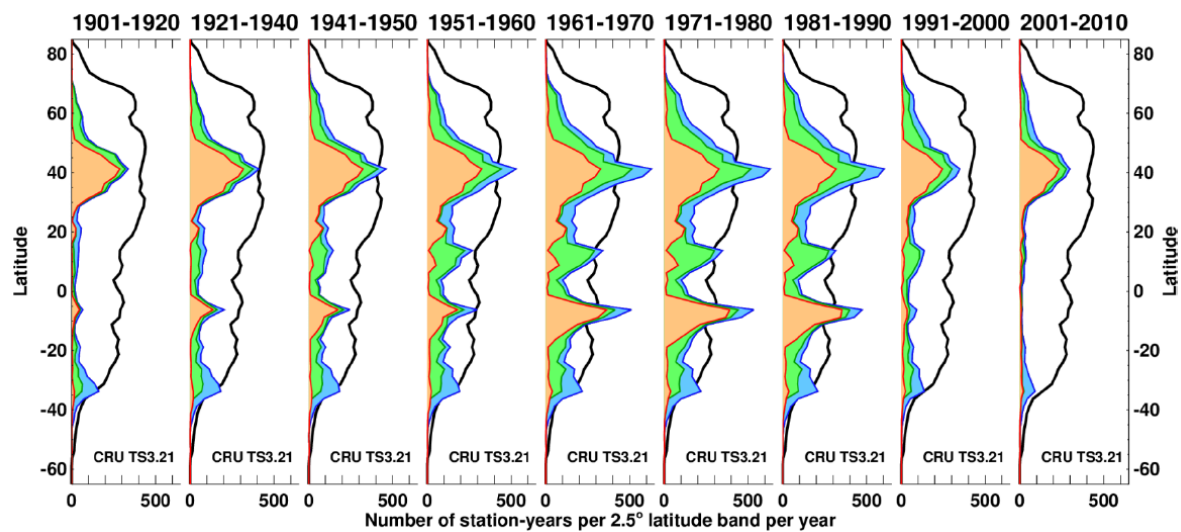
1177 Figure 4: Number of in situ stations over time for the CRU TS 3.21 gridded precipitation 1178 dataset (updated from Harris et al., 2013). Evolution over decades of the latitudinal 1179 density of stations per zonal band for the Americas (orange), Europe/Africa (green) and 1180 Asia/Australasia (blue), stacked to indicate the zonal total. Incomplete data series are 1181 included as a fraction of available data. The black line indicates the number of stations 1182 per zonal band required to obtain an average zonal coverage of 1 station per (100\text{km})^2 1183 of land at that latitude. This figure shows the station numbers in absolute terms and in 1184 relation to the latitudinally-varying land area. Other datasets have similar differences in 1185 coverage over time (see supplementary figure 2 for GPCC). 1186
