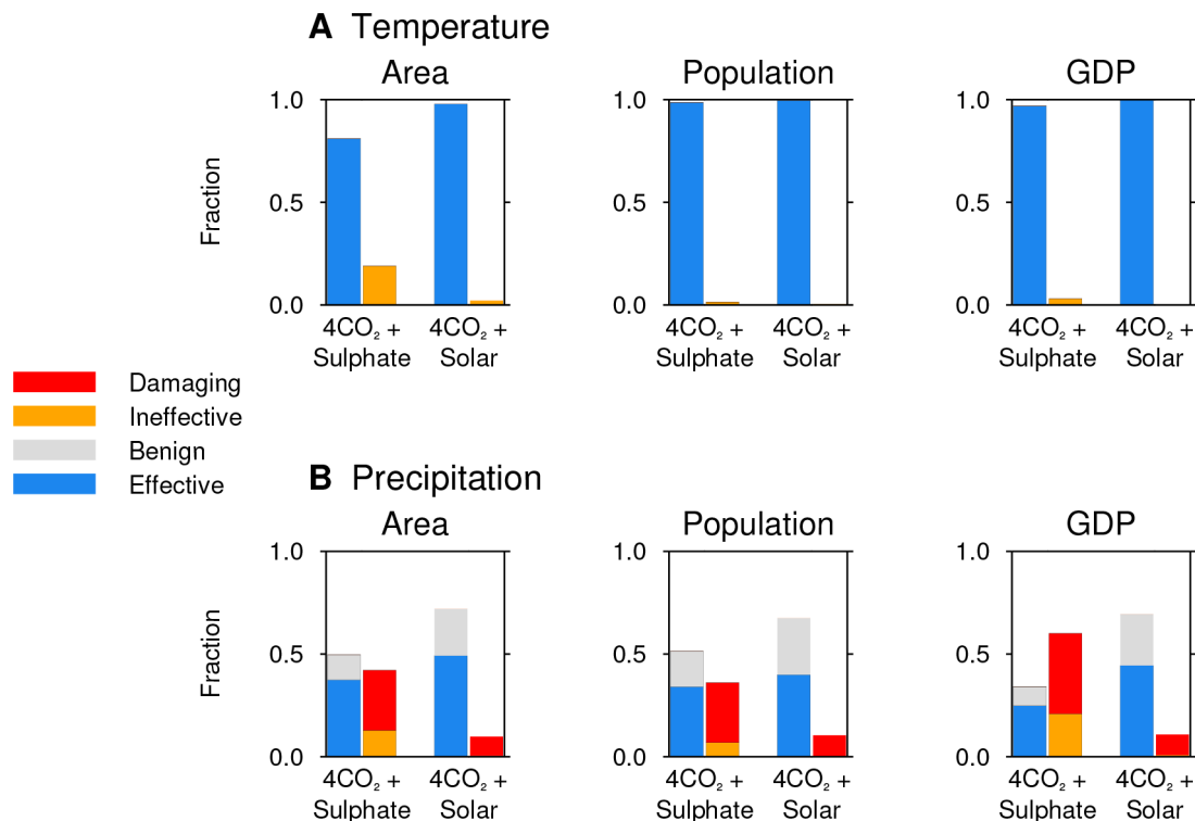
Figure 3. Fraction of global area, population and GDP affected by different outcomes of geoengineering. Each climate model simulation has a pair of bars. The left-hand bar shows the 'benign' and 'effective' outcomes, i.e. where geoengineering reduces risk. The right-hand bar shows the 'damaging' and 'ineffective' outcomes, i.e. where geoengineering increases risk. Regions where neither the response to 4\text{CO}_2 or geoengineering are statistically significant at the 95% level are neglected, so the bars do not sum to 1.0. doi:10.1371/journal.pone.0088849.g003
