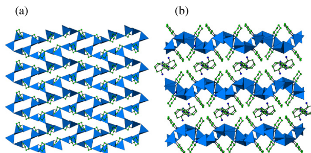
Figure 4: View of (a) a layer of (2) along [301] , and (b) the crystal structure of (2) along [010] .
