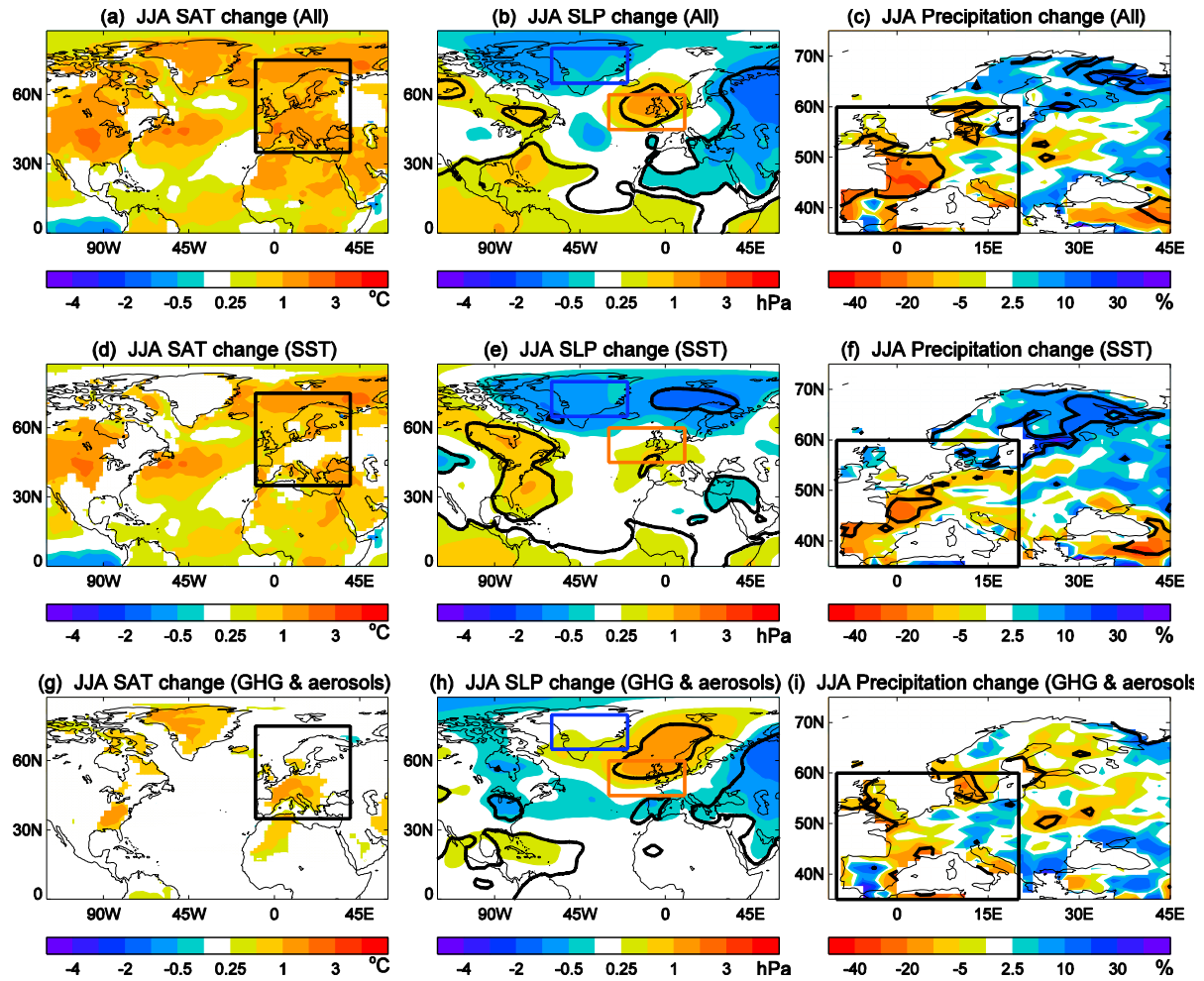
FIGURE. 2. SAT (°C) (left column), SLP (hPa) (middle column) and precipitation changes (%) in the model simulations forced by different configurations of forcings in 2013 relative to the control simulation. (a), (b) and (c) forced by changes in SST and SIE, GHG concentrations, and aerosols emissions (ALL2013-CONTROL). (d), (e) and (f) forced by changes in SST and SIE (SST2013-CONTROL). (g), (h) and (i) forced by changes in GHG and aerosols emissions (ALL2013-SST2013). Only changes that are statistically significant at the 90% confidence level using a two-tailed Student t-test are plotted in (a), (d) and (g) while thick lines in other panels highlight regions where the differences are statistically significant at the 90% confidence level.
