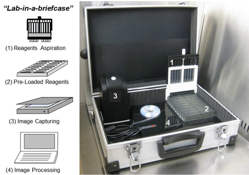
Figure 1. Main components of “Lab-in-a-briefcase” for PSA screening.
