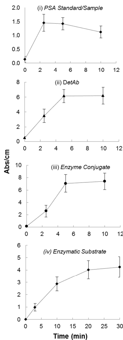
Figure 3. Kinetic study of all assay steps illustrating minimum incubation times required for signal saturation with 3.75 ng/ml of PSA recombinant protein.
