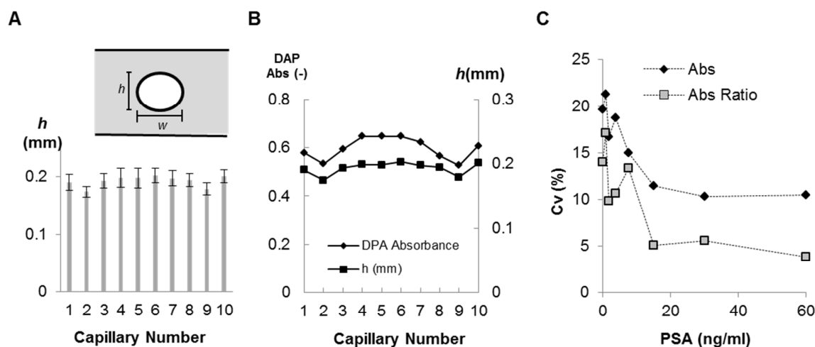
Figure 2. Correlation between capillary height ( h ) and absorbance ( Abs ) variability across a 10 bore fluoropolymer MCF material. A Variation in h across and along the MCF strip (error bars represent 2 standard deviations from multiple measurements along 1m long MCF strip). B Correlation between h and DAP absorbance. C Coefficient of Variation (CV) of absorbance values for different PSA concentration, before and after normalisation with DAP absorbance; CV is obtained from the ratio between the Relative Standard Deviation (STDEV) absorbances along 10 capillaries for a given PSA concentration and the mean value of absorbance in the same 10 capillaries.
