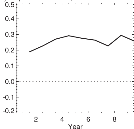
(c) Estimated volcanic forcing error
