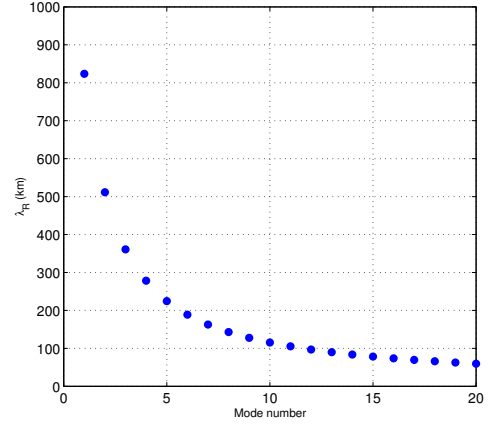
Figure 1. Rossby radius of deformation \lambda_{Rk} for k = 0, \dots, 20 .
