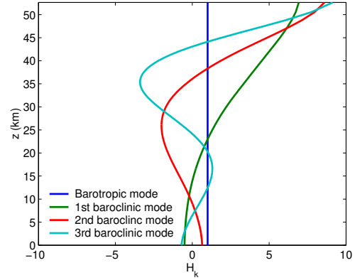
Figure 2. The vertical structure of the barotropic and the first three baroclinic modes.
