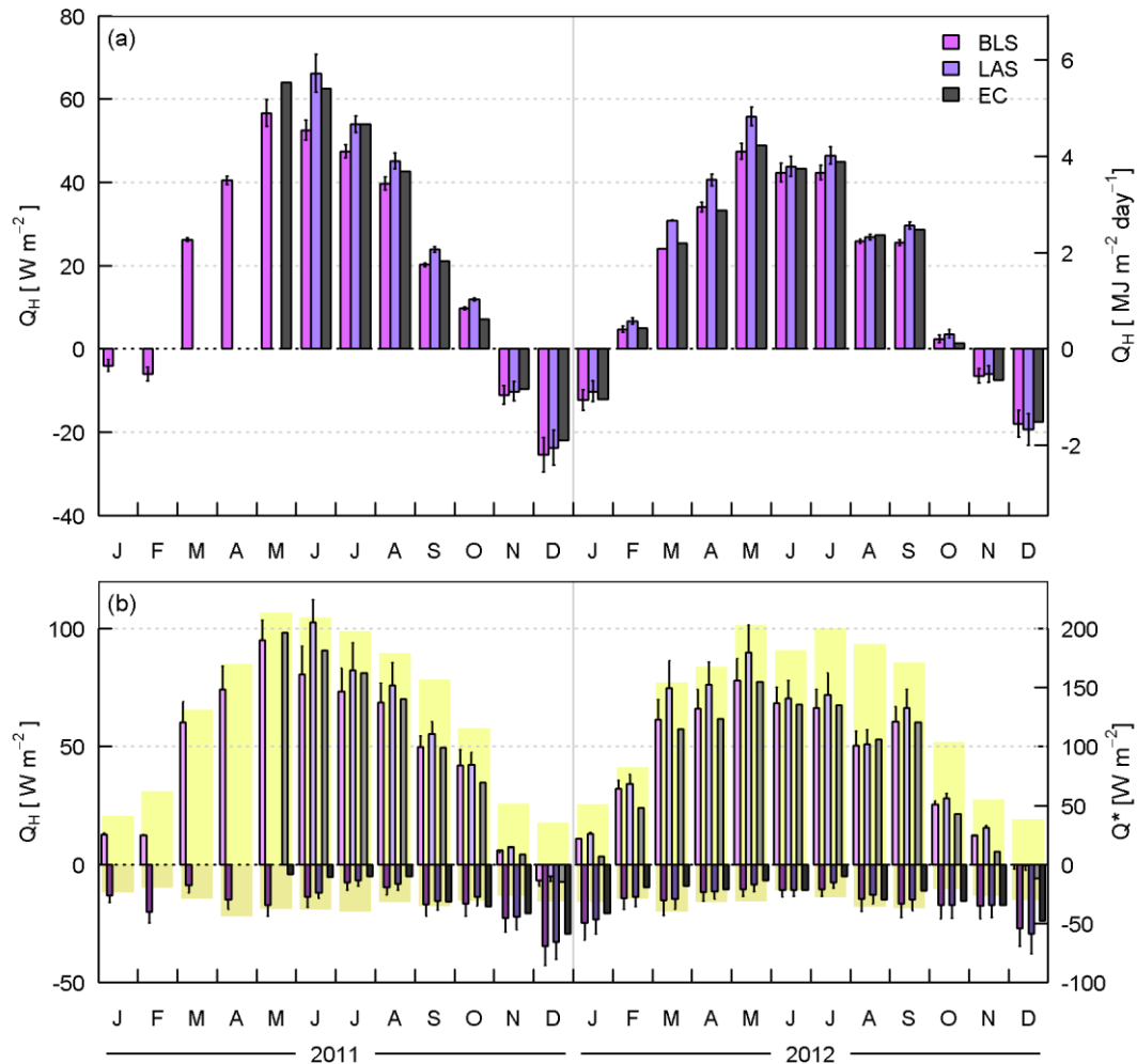
Fig. 3 Monthly mean sensible heat flux observations from scintillometry (BLS and LAS) and eddy covariance (EC) for all available data (a) over 24 h and (b) separated into day ( K_t > 5 \text{ W m}^{-2} ) and night times. Partial months in relation to the installation dates (Table 1) are January 2011 (BLS), May 2011 (EC) and June 2011 (LAS, note only 4 days of data due to an instrument fault). Error bars indicate the impact on the scintillometer fluxes of altering the input roughness length by \pm 0.2 \text{ m} (a) or using the similarity functions of De Bruin et al. (1993) (b). The net radiation is indicated by shading (b, right-hand axis).
