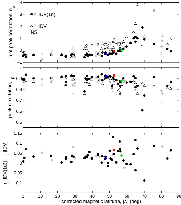
Fig. 3. Analysis of the correlations between IDV(1d) and IDV and BV^n as a function of corrected geomagnetic latitude, \Lambda . In all three panels, open triangles are for IDV, filled circles are for IDV(1d) and black and grey for the Northern and Southern (magnetic) Hemisphere stations, respectively. Results for Eskdalemuir, Neimegk and Nurmijärvi are shown in red, blue and green dots, respectively. (Top) The exponent of V giving the peak correlation, n_p ; (middle) the peak correlation coefficient, r_p ; and (bottom) the difference between r_p for IDV(1d) and IDV.
