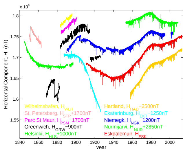
Fig. 1. Daily means of the horizontal component of the field, H , measured at the observatories listed in Table 1: red is Eskdalemuir, ESK; blue is Niemegk, NGK; green is Helsinki, HLS and (after 1952) Nurmijärvi, NUR; orange is Hartland, HAD; mauve is Parc St Maur, PSM; cyan is Ekaterinburg, EKT; black is Greenwich, GRW; yellow is Wilhelmshafen, WLH and pink is St Petersburg, SPE. Note that offsets have been introduced to reduce the y scale needed to display all the data.
