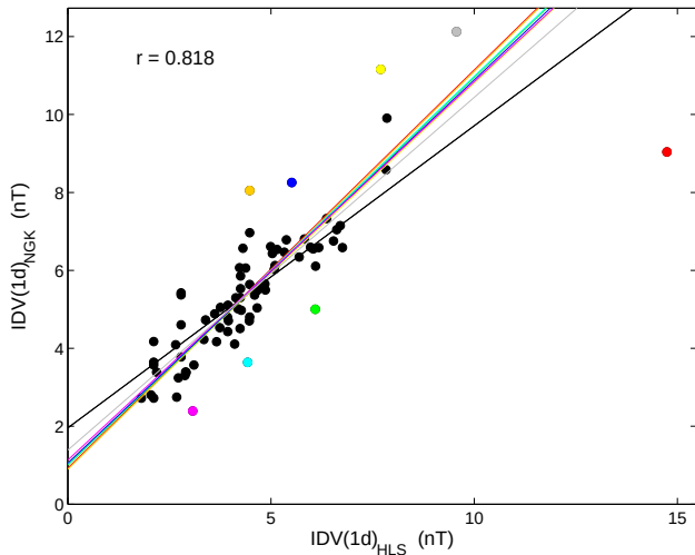
Fig. 6. Scatter plot of Bartels rotation interval means of IDV(1d) values from Helsinki and Niemegk, IDV(1d) HLS and IDV(1d) NGK respectively, for 1890–1897. The coloured dots show outliers removed in the order red, orange, yellow, green, cyan, blue, mauve, and grey. The black line is the regression for no outlier removal and the red line the regression after removal of the red point, and so on. The regression was considered not greatly influenced by outliers after N_r = 4 outliers were removed out of the total of 80 available data points. The correlation coefficient prior to removals was r = 0.818 .
