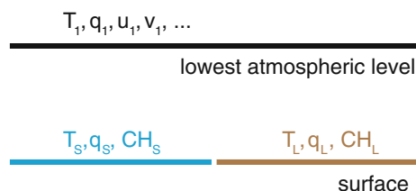
Fig. 9 Schematic of the coastal tiling scheme. At surface level, the model grid-box is divided into a land and a sea part, with pertinent variables such as temperature T and specific humidity q , and also exchange coefficients CH . No distinction between land and sea is made at the lowest atmospheric level
