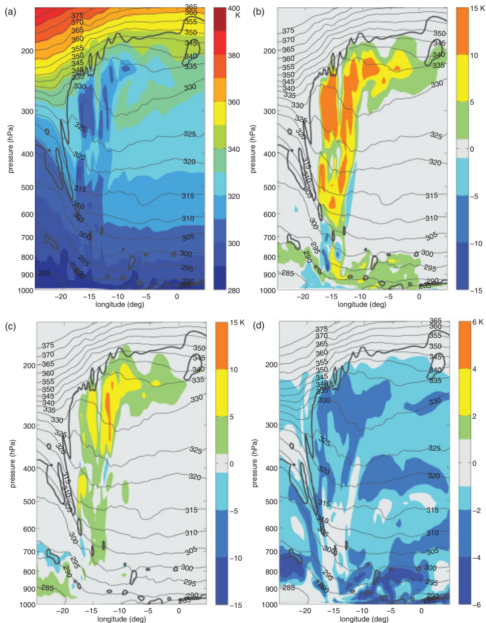
Figure 7. Vertical section along the segment AB indicated in Figure 3 for 0600 UTC on 30 September 2011 showing (a) \theta_0 , (b) \Delta\theta_{\text{LSlh}} , (c) \Delta\theta_{\text{conv}} and (d) \Delta\theta_{\text{rad}} . Note the different colour scales used. Bold black lines represent the 2 PVU contour. Thin black lines represent potential temperature contours with a 5 K separation.
