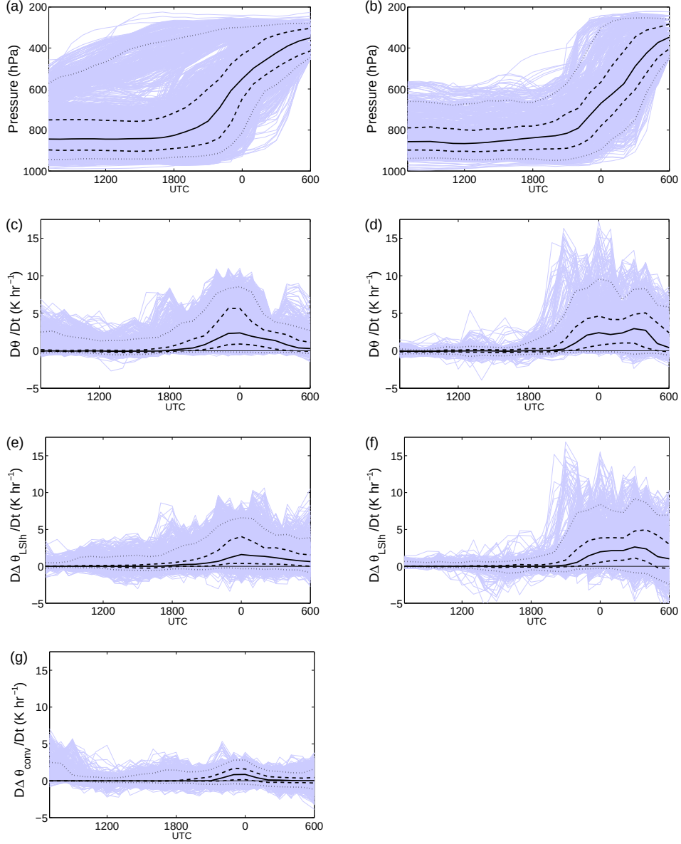
Figure 11: Evolution along trajectories of (a,b) pressure, in hPa, (c,d) D\Delta\theta/Dt , (e,f) D\Delta\theta_{LSih}/Dt and (g) D\Delta\theta_{conv}/Dt for the simulations STDCON (left column; panels a, c, e and g) and REDCON (right column; panels b, d and f). In each case the solid lines represent the median; dashed lines represent the 25th and 75th percentiles; and, dotted lines represent the 5th and 95th percentiles of the trajectory ensemble. Light grey lines represent individual trajectories within the ensemble.
