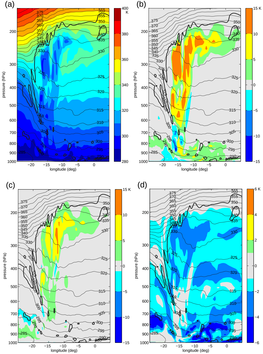
Figure 7: Vertical section along the segment AB indicated in Figure 3 for 0600 UTC 30 September 2011 showing (a) \theta_0 , (b) \Delta\theta_{\text{LSlh}} , (c) \Delta\theta_{\text{conv}} and (d) \Delta\theta_{\text{rad}} . Note the different colour scales used. Bold black lines represent the 2-PVU contour. Thin black lines represent potential temperature contours with a 5-K separation.
