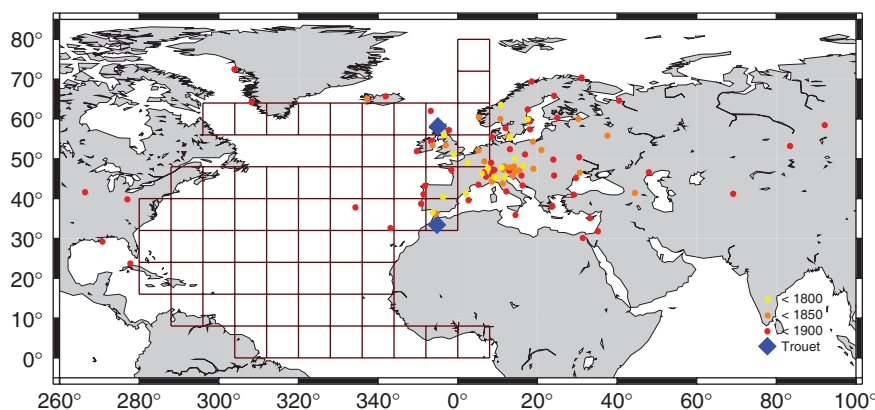
FIGURE 4 An example of the location of proxy records used to reconstruct the NAO index: in blue the precipitation sensitive proxy locations used in Trouet et al., 6 in yellow to dark red the proxy locations (only pressure sensitive) used in the MSLP reconstruction of Kuettel et al. 79 Note that the proxy records of Trouet et al. 6 span the period 1000–1995, whereas the proxy records of Kuettel span different periods; the red boxes are 8^\circ \times 8^\circ grid boxes sampling wind speed and direction derived from ship log books from 1662 to 1855, 81 where 99.6% span the period from 1750 to 1855. 79
