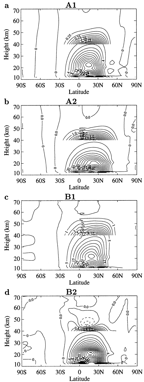
FIG. 3. As in Fig. 2 but for the TEM streamfunction. Contour intervals below and above 40 km are (a) 2 and 0.25 \text{ kg m}^{-1} \text{ s}^{-1} , (b) 10 and 0.5 \text{ kg m}^{-1} \text{ s}^{-1} , (c) 5 and 1 \text{ kg m}^{-1} \text{ s}^{-1} , and (d) 2 and 0.2 \text{ kg m}^{-1} \text{ s}^{-1} . Positive values denote a circulation in the clockwise sense.
