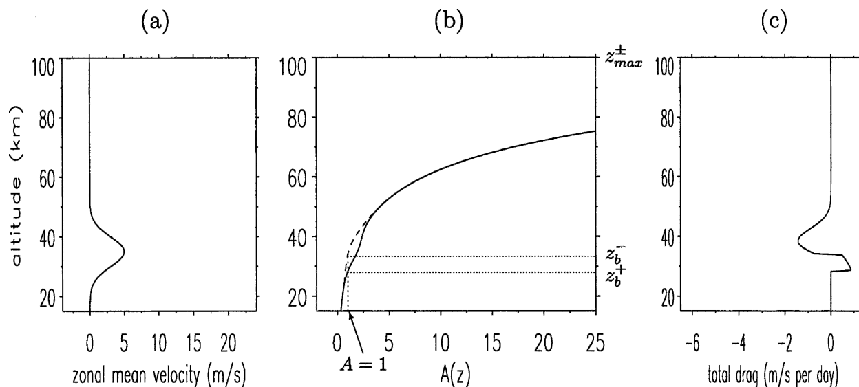
FIG. 4. Lindzen parameterization with two waves with phase speeds c^\pm = \pm 25 \text{ m s}^{-1} . (a) Initial mean velocity with maximum value of \bar{u}_{\max} = 5 \text{ m s}^{-1} , (b) the function A^\pm(z) defined in (3.1), and (c) the total drag from the two waves.
