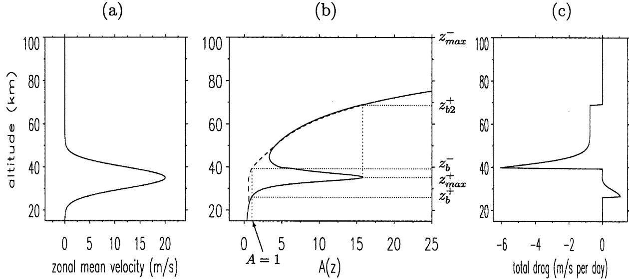
FIG. 2. Lindzen parameterization with two waves with phase speeds c^\pm = \pm 25 \text{ m s}^{-1} . (a) Initial mean velocity with maximum value of \bar{u}_{\max} = 20 \text{ m s}^{-1} , (b) the function A^\pm(z) defined in (3.1), and (c) the total drag from the two waves.
