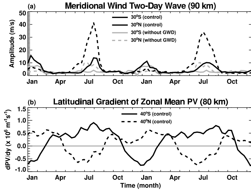
Figure 6. Time series of (a) the amplitude of the meridional wind component of the 2-day wave ( m = -3 ; 0.4 \leq \omega \leq 0.8 cpd) at 30^\circ\text{N/S} , 90 km, and (b) the latitudinal derivative of the zonal mean PV at 40^\circ\text{N/S} , 80 km. The black lines denote the control simulation; the shaded lines in Figure 6a are for the 1-year simulation without nonorographic GWD for which the second year is repeated. Results are computed using a 20-day window.
