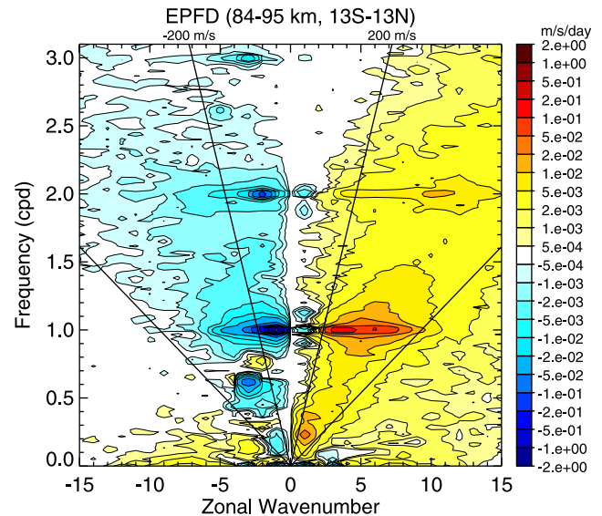
Figure 12. Annual mean zonal wavenumber ( m ) and frequency ( \omega ) spectrum of \nabla \cdot \vec{F}/(\rho_0 a \cos \phi) averaged from 13°S to 13°N and from 84 to 95 km for the control simulation. The spectral peak at m = -1 and \omega = 1 cpd is the migrating diurnal tide; |m| < 8 ( m \neq -1 ) and \omega = 1 cpd are nonmigrating diurnal tides. The two unlabeled diagonal lines denote the plus and minus 50 m/s phase speeds. See Figure 4 caption for more details.
