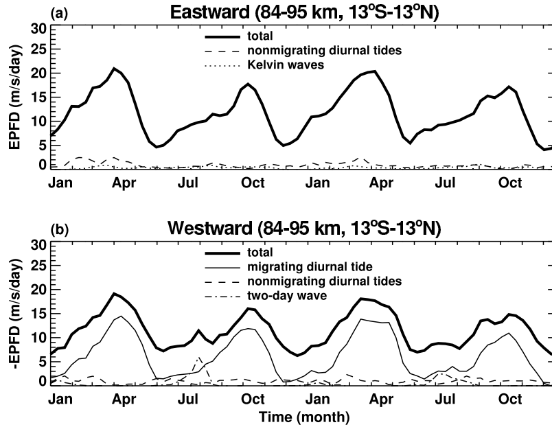
Figure 13. Time series of \nabla \cdot \vec{F}/(\rho_o a \cos \phi) averaged from 13°S to 13°N and from 84 to 95 km for the control simulation: (a) eastward and (b) westward traveling disturbances. The wave types are defined as nonmigrating diurnal tides ( |m| = 1-5 ( m \neq -1 ), \omega = 1 cpd), migrating diurnal tide ( m = -1 , \omega = 1 cpd), Kelvin waves ( m = +1-5 , \omega \leq 0.3 cpd), and 2-day wave ( m = -3 , 0.4 \leq \omega \leq 0.8 cpd). The thick solid lines denote the sum of all wavenumbers and frequencies for each direction. Results are computed using a 20-day window.
