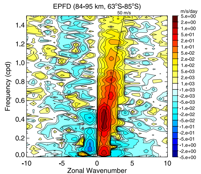
Figure 7. Zonal wavenumber ( m ) and frequency ( \omega ) spectrum of \nabla \cdot \vec{F}/(\rho_0 a \cos \phi) averaged from 63^\circ\text{S} to 85^\circ\text{S} and from 84 to 95 km for June, July, and August of the control simulation. The broad spectral peak centered at m = +1 and \omega \sim 0.4 cpd is the 4-day wave. See Figure 4 caption for more details.
