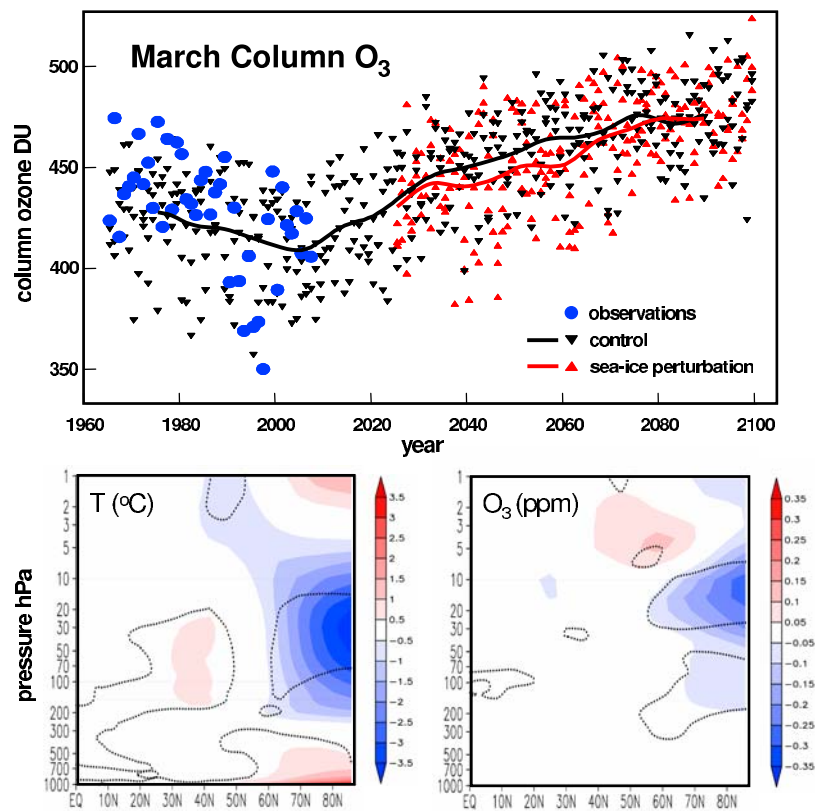
Figure 2. (top) Time series of Arctic springtime column ozone (averaged over 60°N–90°N and the month of March) from observations (updated from Fioletov et al. [2002], large blue dots), the CMAM control ensemble (black triangles and thick black line), and the average over the CMAM ensemble in which sea-ice was perturbed beginning in 2025 (red triangles and thick red line). Thick lines are derived from a running mean over the ensemble average employing a Gaussian window with a half-width of 10 years. Northern Hemisphere March anomaly (sea-ice perturbation minus control) of (bottom left) temperature and (bottom right) ozone mixing ratio averaged over 2040–2060, ensemble members, and longitude. Dotted contour lines indicate significance at the 95% confidence level.
