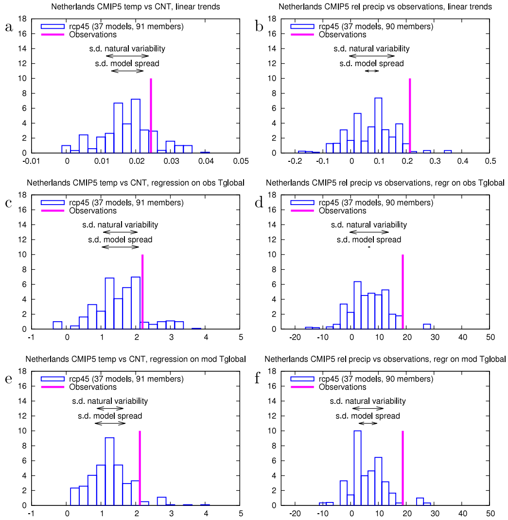
Figure 1. (a) Trend in the homogenized central Netherlands temperature over 1950–2011 compared to the CMIP5 ensemble interpolated to 52^\circ\text{N} , 5^\circ\text{E} using a linear trend definition ( \text{K yr}^{-1} ). (b) Same for the homogenized Netherlands precipitation ( \text{\% yr}^{-1} ). (c, d): As (a, b) but with the trend defined as the regression on the low-pass filtered observed global mean temperature, equation (2) ( \text{K K}^{-1} ), ( \text{\% K}^{-1} ). (e, f): As (c, d) but using the modelled global mean temperature, equation (3).
