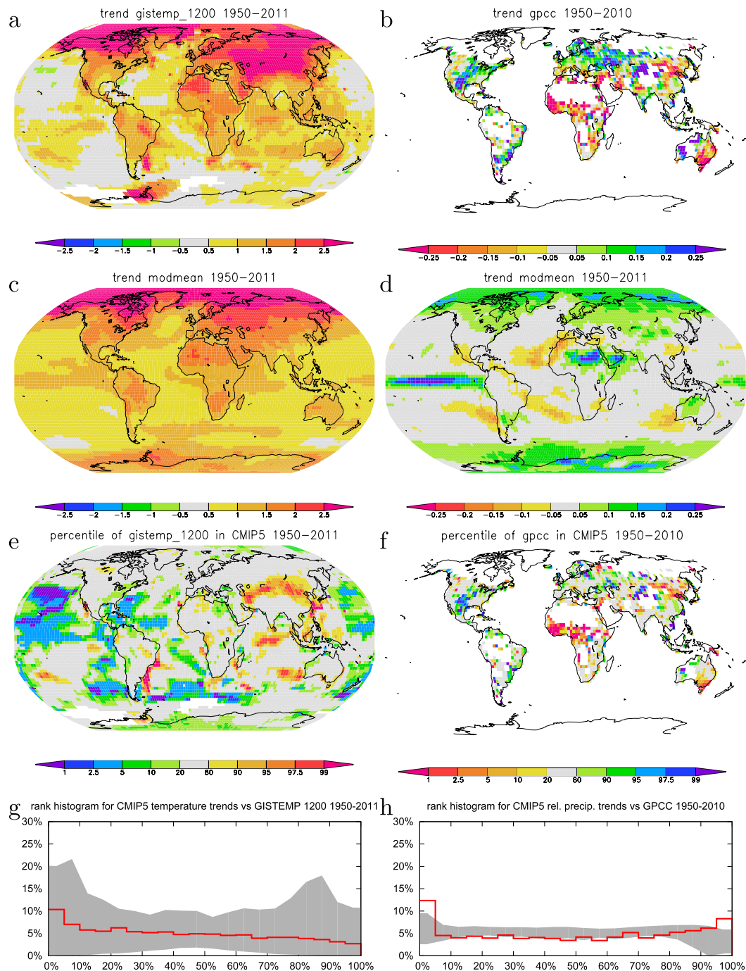
Figure 2. Observed trends 1950–2011 in (a) GISTEMP temperature (decorrelation scale 1200 km) ( \text{K K}^{-1} ) and (b) GPCC precipitation ( \text{\% K}^{-1} ) as regression on the observed global mean temperature equation (2) (white areas do not have enough data to compute a trend); (c, d) corresponding CMIP5 multi-model mean trends; (e, f) percentile of the observed trends in the CMIP5 ensemble at the same grid point; (g, h) red line: rank histograms of GISTEMP temperature and GPCC precipitation trends versus the CMIP5 trends north of 45^\circ\text{S} , grey area: the 90% range obtained from the inter-model variations.
