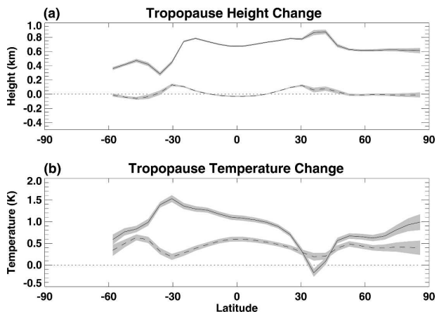
FIG. 16. Change in (a) tropopause height (km) and (b) tropopause temperature (K) induced by the CO 2 doubling with (solid curves, experiments C2–B1) and without (dashed curves, experiments B2–B1) changes in SSTs taken into account. The data shown are zonal and annual mean values averaged over 30 yr. The shading represents the standard error of the difference between the means.
