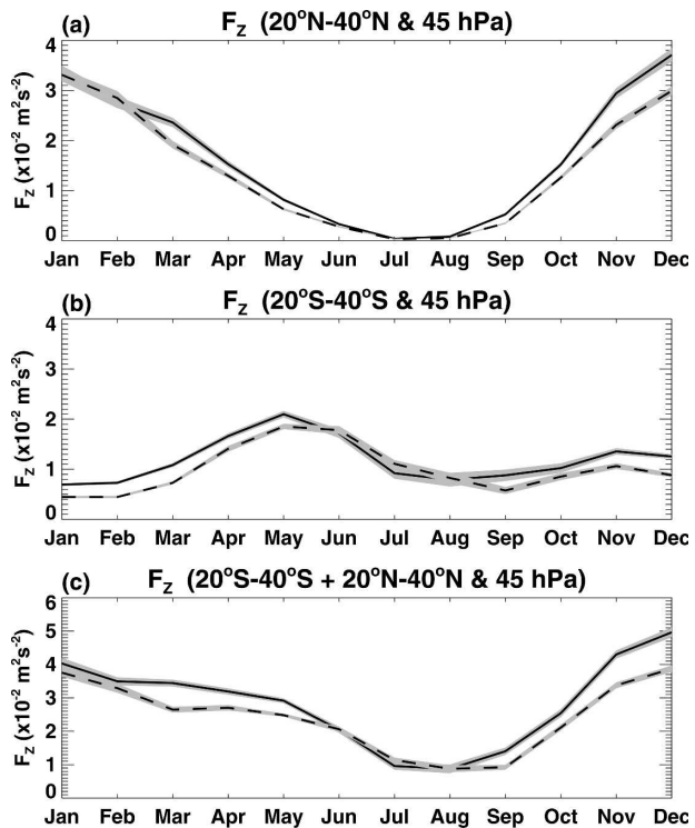
FIG. 19. Annual cycle of the vertical component of the EP flux ( 10^{-2} \text{ m}^2 \text{ s}^{-2} ) at 45 hPa ( \sim 22 \text{ km} ) for experiments C2 (solid, 2\times\text{CO}_2 with modified SSTs) and B1 (dashed, control experiment) averaged from (a) 20^{\circ} – 40^{\circ}\text{N} , (b) 20^{\circ} – 40^{\circ}\text{S} , and (c) 20^{\circ} – 40^{\circ}\text{N} and 20^{\circ} – 40^{\circ}\text{S} . The data shown are zonal and monthly mean values averaged over 30 yr. The shading represents the standard error of the mean. [Here F_z is equivalent to F_z/(a\rho_0) used by Andrews et al. (1987) in Eq. (3.5.3), p. 128.]
