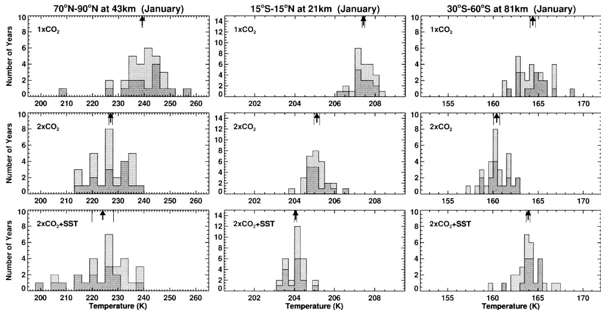
FIG. 15. Histograms of latitudinally averaged zonal mean temperature for (left) January at 70°–90°N, 43 km; (middle) 15°S–15°N, 21 km; and (right) 30°–60°S, 81 km for (top row) 1 \times CO 2 (experiment B1); (middle row) 2 \times CO 2 (experiment B2); and (bottom row) 2 \times CO 2 with modified SSTs (experiment C2). The dark shading denotes data from the second 15-yr subset (subset S 2 ); the combined light and dark shading denote the full 30-yr dataset. The arrow at the top denotes the mean of the 30-yr dataset; the two thin lines on either side are the means of the respective 15-yr subsets.
