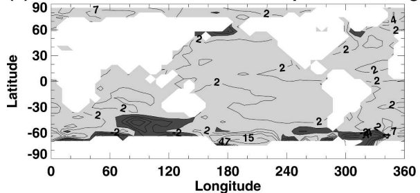
FIG. 1. Seasonal mean change in the marine surface temperature (prescribed sea surface temperature and calculated sea ice temperature) in the 2\times\text{CO}_2 climate compared to the control experiment B1. (a) December–February. The large change in the Arctic reflects the fact that there is no sea ice in the 2\times\text{CO}_2 climate. (b) June–August. Contours are 0, \pm 2 , \pm 4 , \pm 7 , \pm 15 , and 30 K. Dark shading is applied to regions with negative values.
