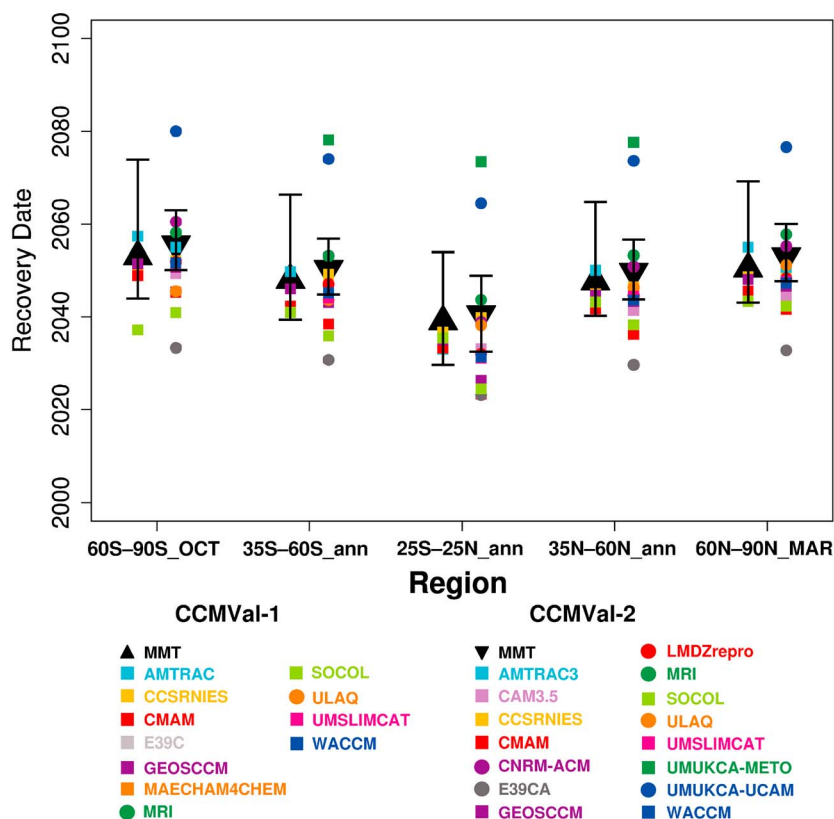
Figure 13. Date of return to 1980 values for the annual average 50 hPa \text{Cl}_y , derived from the IMT (colored symbols) and MMT (large black triangles) estimates for CCMVal-1 and CCMVal-2 (left and right entries, respectively, in each latitude band). The error bars on the MMT estimate of return date is derived from the 95% confidence interval of the MMT estimates to the 1980 baseline-adjusted time series data.
