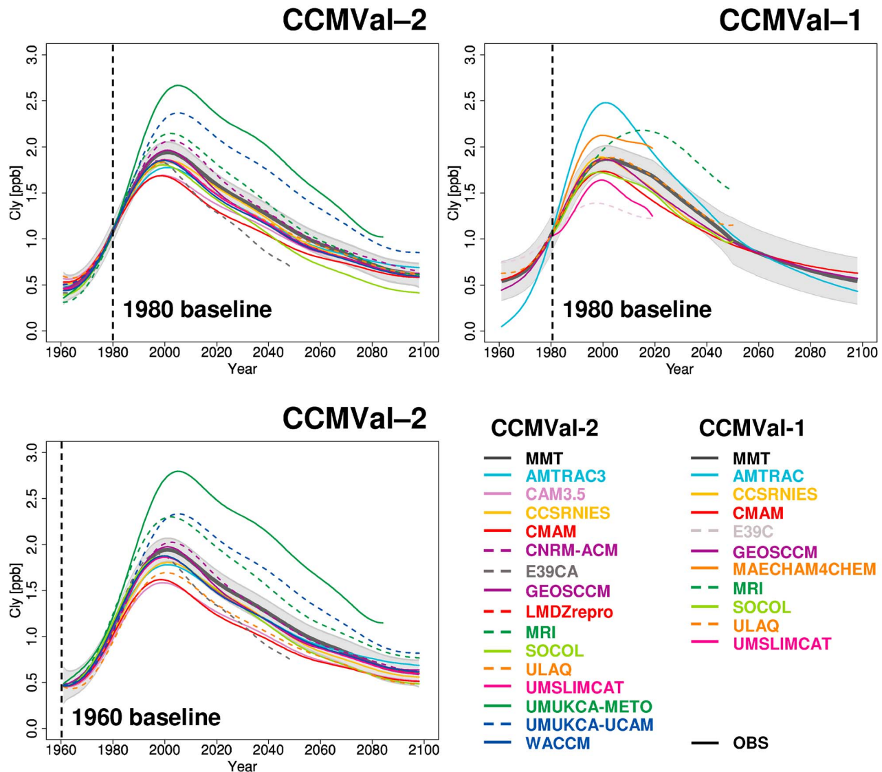
Figure 6. Same as Figure 2 but for 50 hPa \text{Cl}_y in the latitude range 35^\circ\text{N} – 60^\circ\text{N} .
