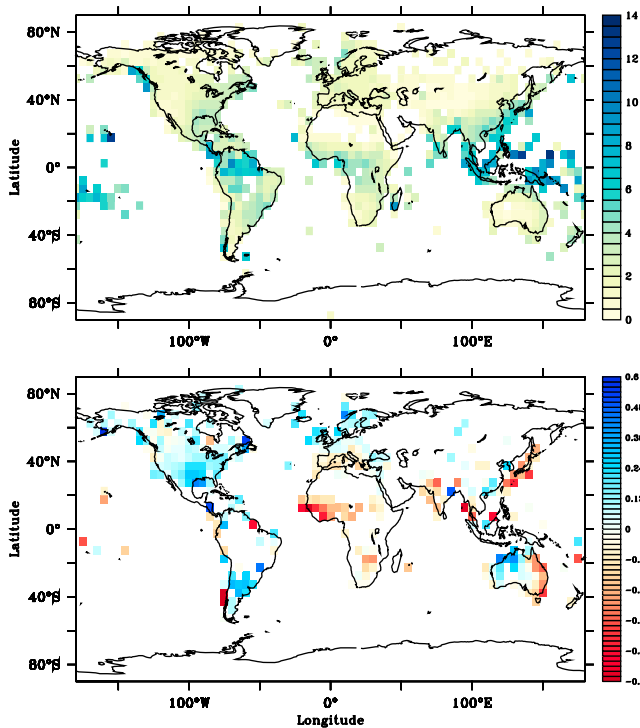
Figure 1. (top) Observed climatological precipitation (mm/day) for the baseline period of 1961–90. (bottom) Spatial map of observed trend (mm/day/yr), for 1951–2005.
