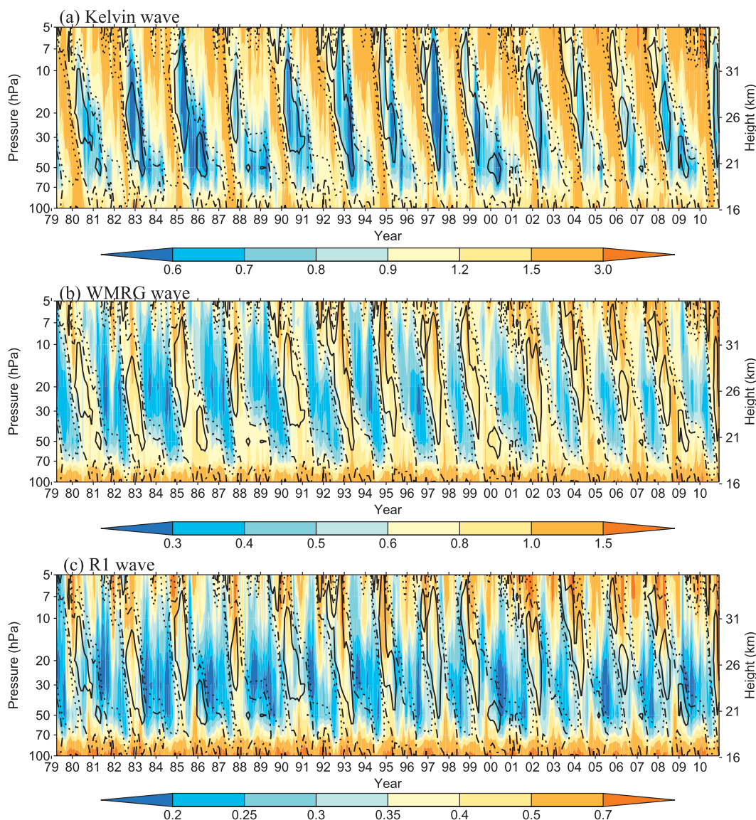
FIG. 5. (a) Time–height cross section of monthly zonal-averaged standard deviations of (a) Kelvin wave equatorial u , (b) WMRG wave equatorial v , and (c) R1 wave v at 8^{\circ}\text{N}/8^{\circ}\text{S} ( \text{m s}^{-1} ). The black solid and dotted contours indicate monthly mean zonal winds of 10 and -10 \text{ m s}^{-1} , respectively, and the dot-dashed contour indicates zero wind.
