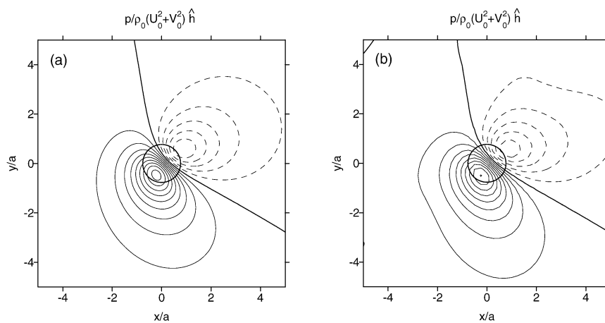
FIG. 6. Normalized total pressure perturbation at the surface for the flow given by (54) when \text{Ri} = 0.5 . (thick solid line) Terrain elevation equal to 0.5h_0 ; (solid contours) positive values; (dashed contours) negative values, contour spacing 0.05. (a) Present model; and (b) NH3D numerical model.
