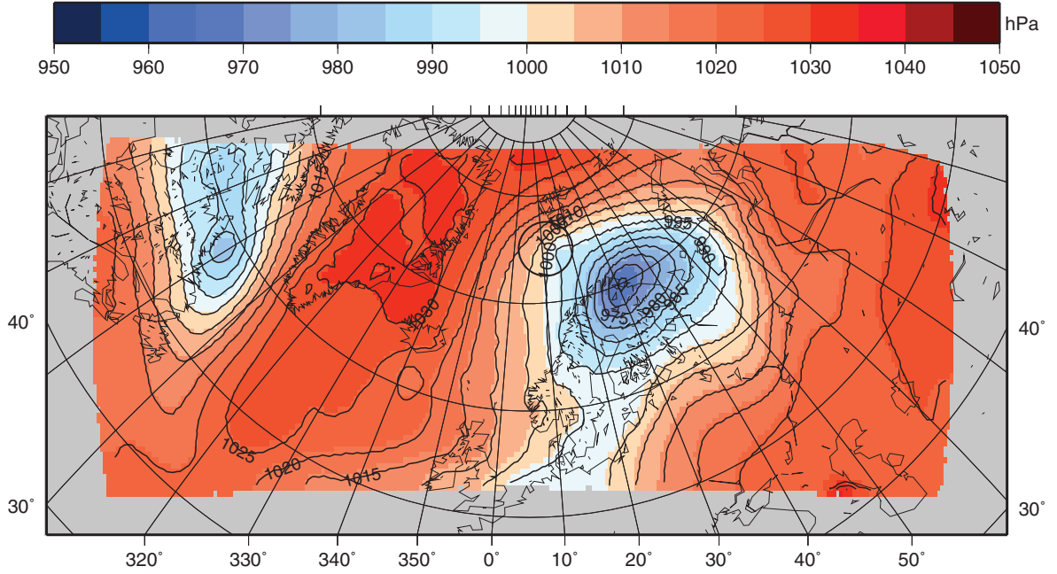
Fig. 1. Unfiltered MSLP field on 06:00 14 October 1993 (hPa).
