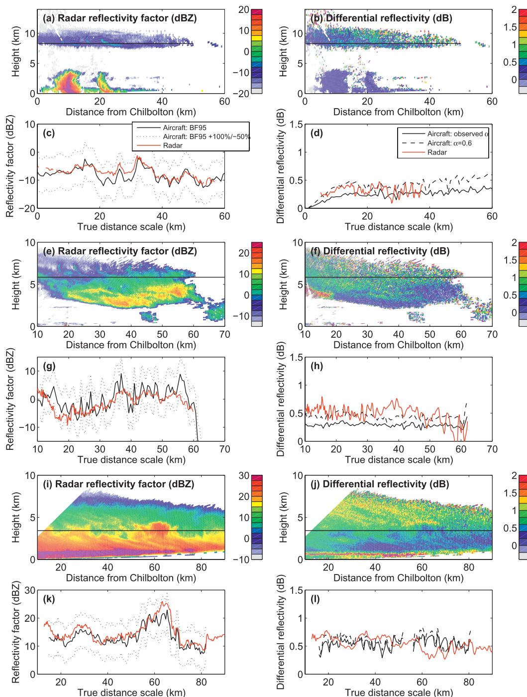
FIG. 6. (a),(b) Radar reflectivity factor Z_h and differential reflectivity Z_{dr} at 1334 UTC 8 Oct 1997, where the horizontal black line indicates the altitude of the aircraft (where the temperature was -32^{\circ}\text{C} ); (c),(d) aircraft-calculated Z_h and Z_{dr} in black [assuming the Brown and Francis (1995) mass-size relationship], with radar measurements in red. The dotted lines in (c) indicate the effect on Z_h of doubling or halving the mass of the particles, and (d) contains two aircraft calculations: one using the measured particle axial ratios, and the other assuming \alpha = 0.6 . (e)–(h) As in (a)–(d), but at 1049 UTC 20 Oct 2000, when the aircraft was sampling at a temperature of -24^{\circ}\text{C} . (i)–(l) As in (a)–(d), but at 1459 UTC 21 Nov 2000, when the aircraft was sampling at -10^{\circ}\text{C} .
