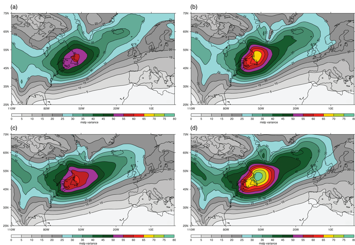
Figure 7. Variance of bandpass 2- to 6-day filtered winter (DJF) MSLP fields for (a) ERA40; (b) HiGEM; (c) HiGAM control and (d) HiGAM perturbed. Units in \text{hPa}^2 .
