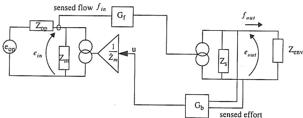
Figure 5. Two port telemanipulator model
