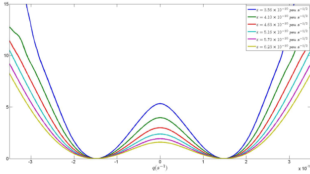
Fig. 2. One-dimensional adimensional potential U(q) obtained as minus the logarithm of the pdf given in Fig. 1.
